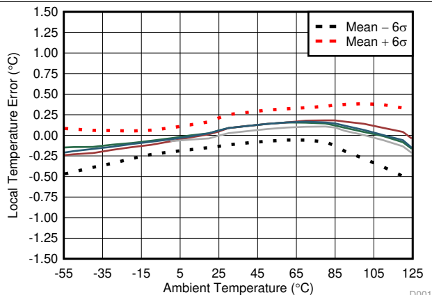
图 2. Local Temperature Error vs Ambient Temperature
