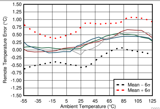
图 3. Remote Temperature Error vs Ambient Temperature
