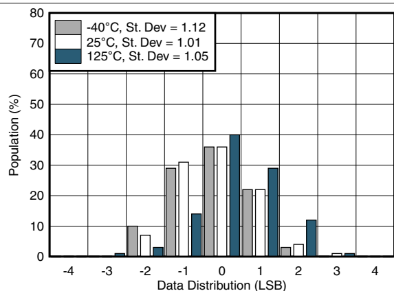
图 6. Data Reading Distribution Over Temperature (No Averaging)
