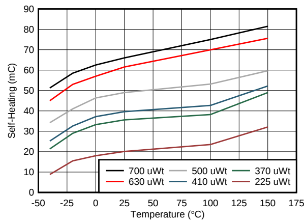
图 43. Self-Heating in Still Air vs. Temperature and Dissipated Power at 25°C
