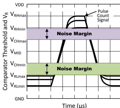
Figure 23. Pulse Count Signal Amplitude Variation
