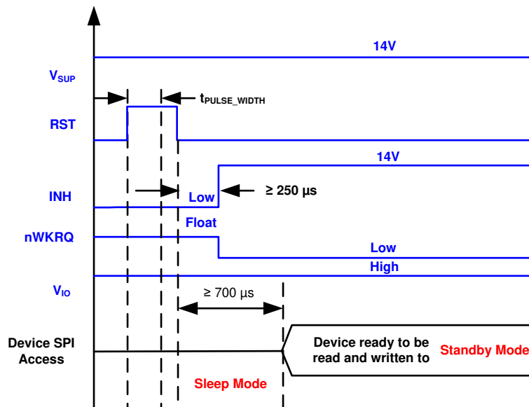
图 8-4. Timing for RST Pin in Sleep Mode
