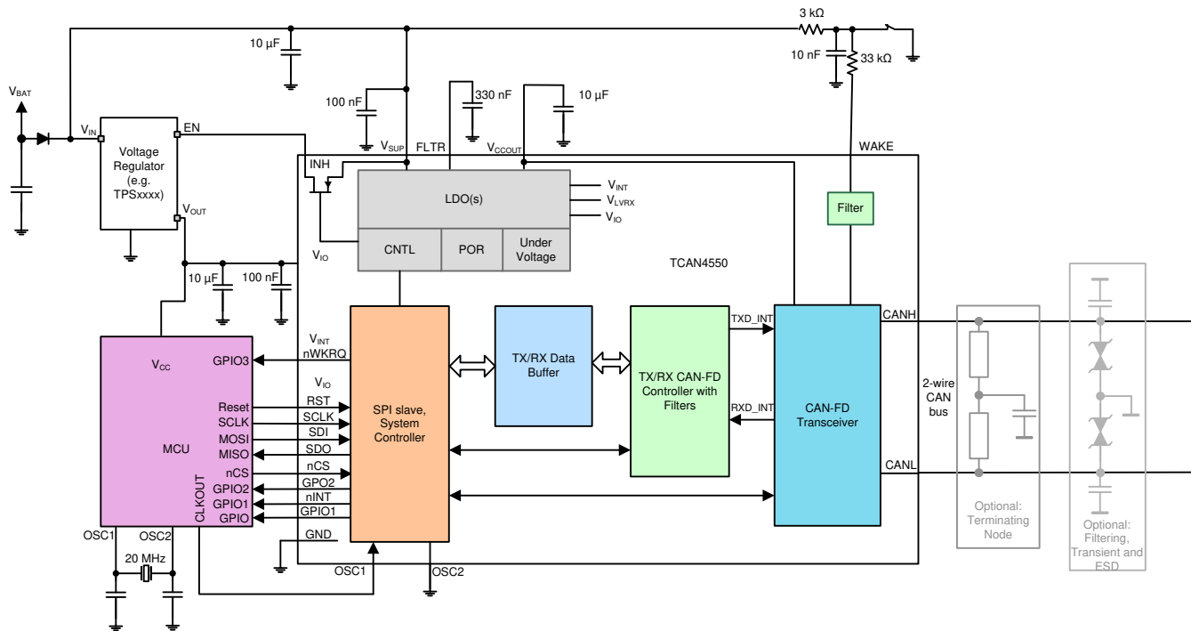
图 9-7. Typical CAN Applications for TCAN4550-Q1 for 3.3 V µC; Clock from MCU
