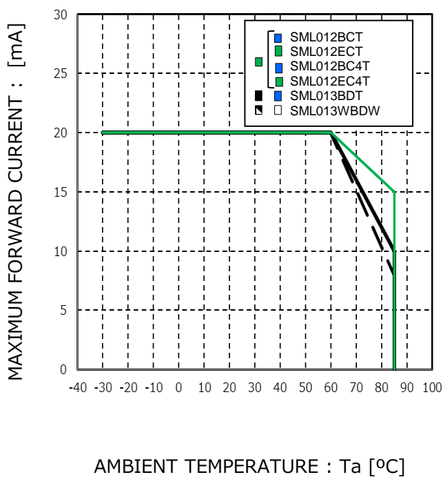
Fig.4 Derating
