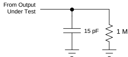
图 4. Load Circuit For Maximum Data Rate: Pulse Duration, Propagation Delay Output Rise, And Fall Time Measurement
