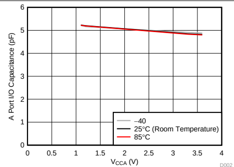
图 2. Capacitance for A port I/O Pins ( C_{IO} ) vs Power Supply ( V_{CCA} )
