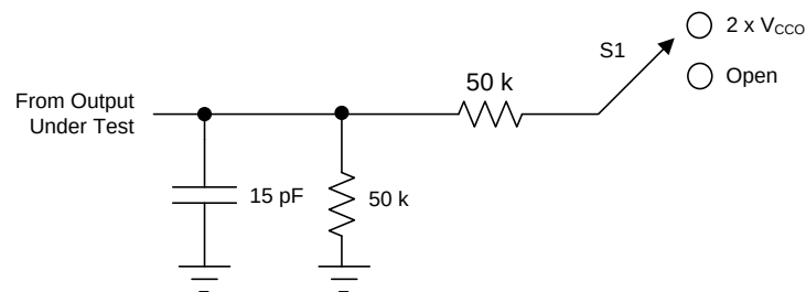
图 5. Load Circuit For Enable / Disable Time Measurement
