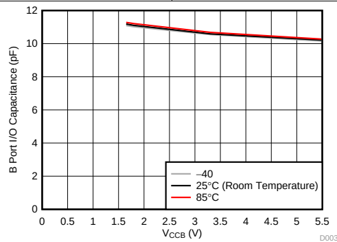
图 3. Capacitance for B Port I/O Pins ( C_{IO} ) vs Power Supply ( V_{CCB} )
