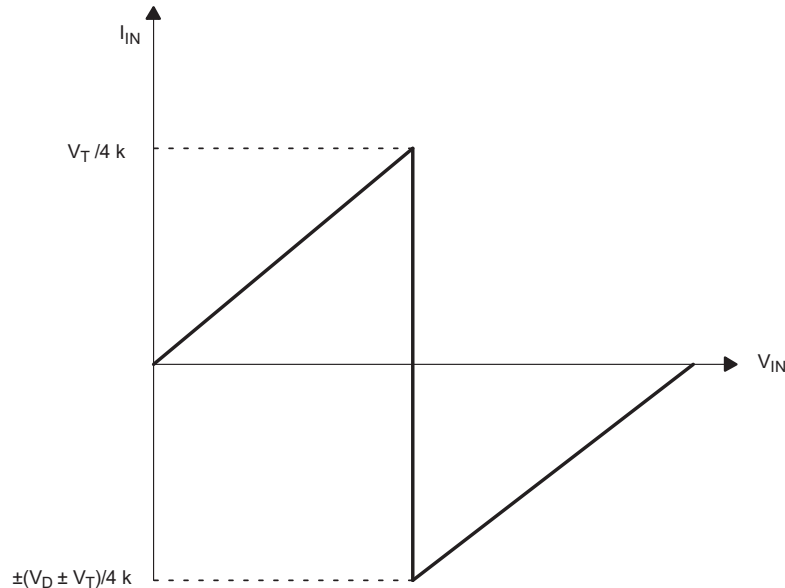
图 9. Typical I_{IN} vs V_{IN} Curve
