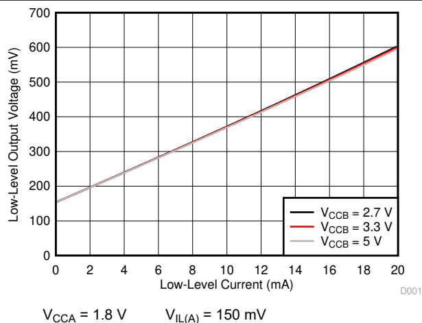
图 6-1. Low-Level Output Voltage ( V_{\text{OL(Ax)}} ) vs Low-Level Current ( I_{\text{OL(Ax)}} )
