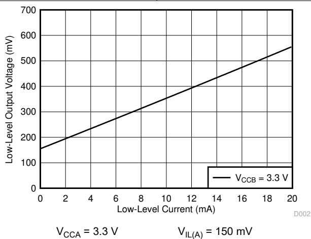
图 6-3. Low-Level Output Voltage ( V_{\text{OL(Ax)}} ) vs Low-Level Current ( I_{\text{OL(Ax)}} )
