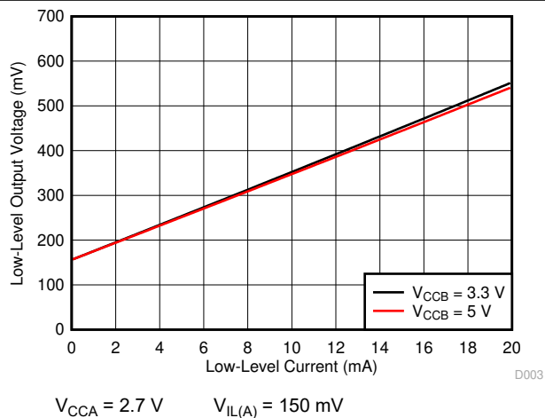
图 6-2. Low-Level Output Voltage ( V_{\text{OL(Ax)}} ) vs Low-Level Current ( I_{\text{OL(Ax)}} )
