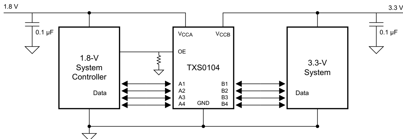
图 9-1. Application Schematic
