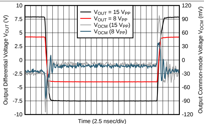
图 10. Pulse Response Drive Mode 2 (Bias Z1)
