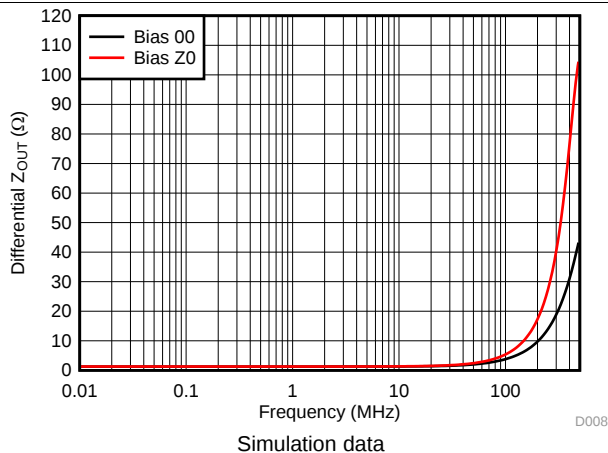
图 8. Termination Mode Differential Output Impedance
