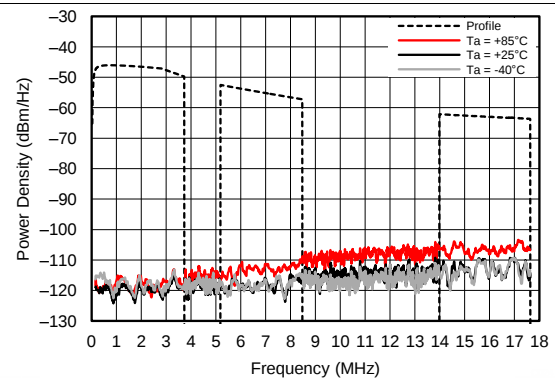
Figure 23. Dual-Channel Profile 8 MTPR vs Temperature
