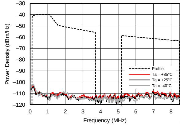
Figure 15. Single-Channel ADSL MTPR vs Temperature
