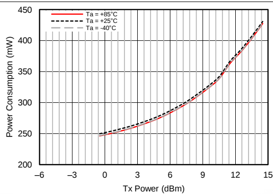
Figure 22. Dual-Channel Profile 8 Power Consumption vs Temperature
