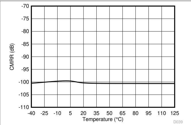
图 6-12. Common-Mode Rejection Ratio vs Temperature
