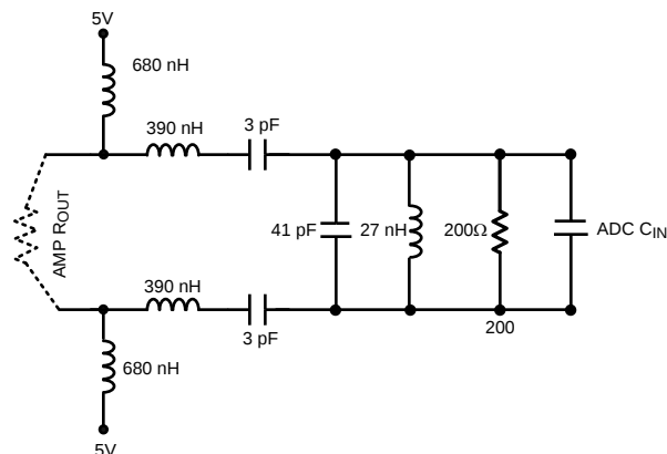
Figure 50. Bandpass Filter
