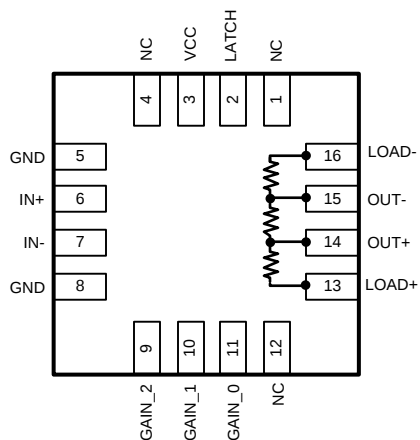
Figure 52. Internal Load Resistors
