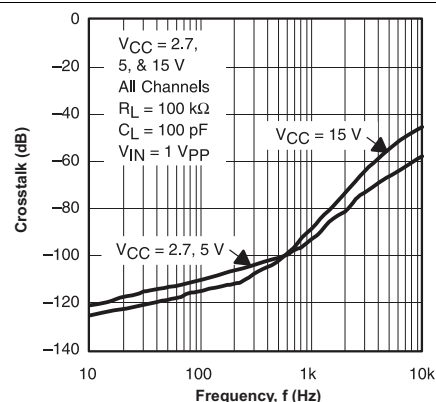
Figure 36. Crosstalk
