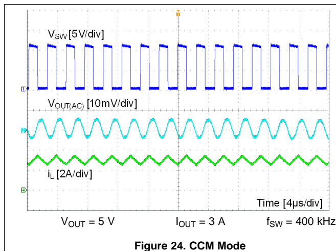
Figure 24. CCM Mode
