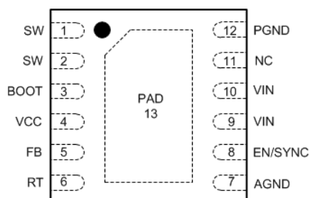
DRR Package 12-Pin WSON With RT and Thermal Pad Top View
