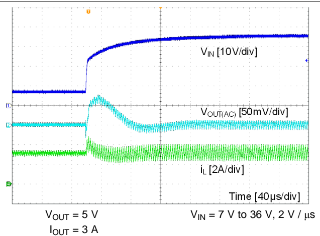
Figure 31. Line Transient
