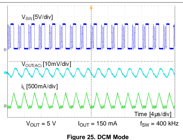
Figure 25. DCM Mode
