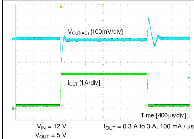
Figure 30. Load Transient
