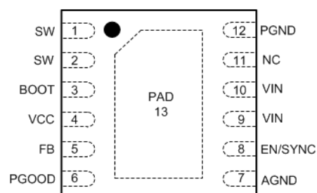
DRR Package 12-Pin WSON With PGOOD and Thermal Pad Top View
