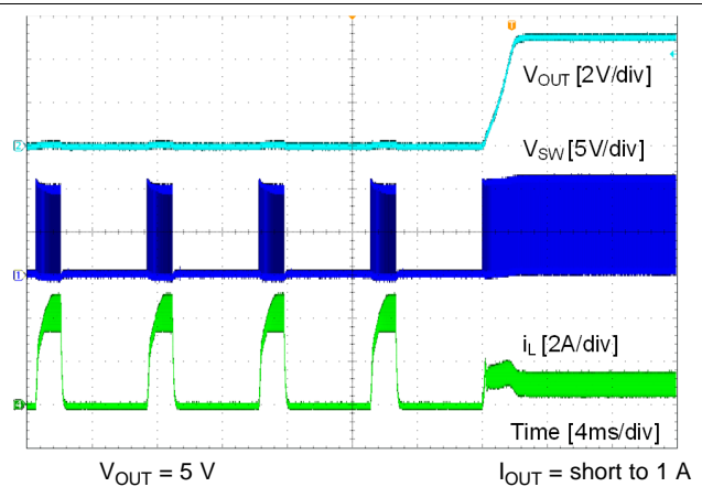
Figure 33. Short Recovery
