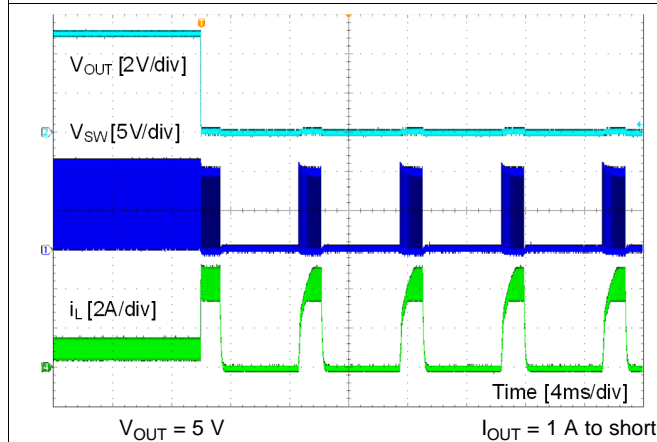
Figure 32. Short Protection
