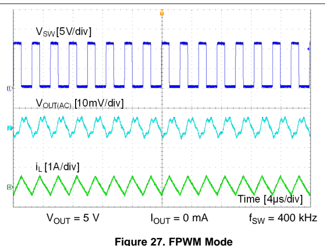
Figure 27. FPWM Mode
