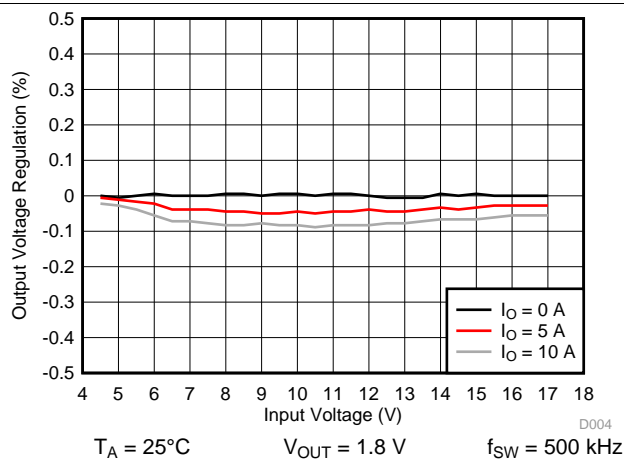
图 41. Line Regulation
