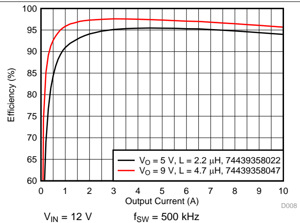
图 2. Efficiency With 5-V and 9-V Output
