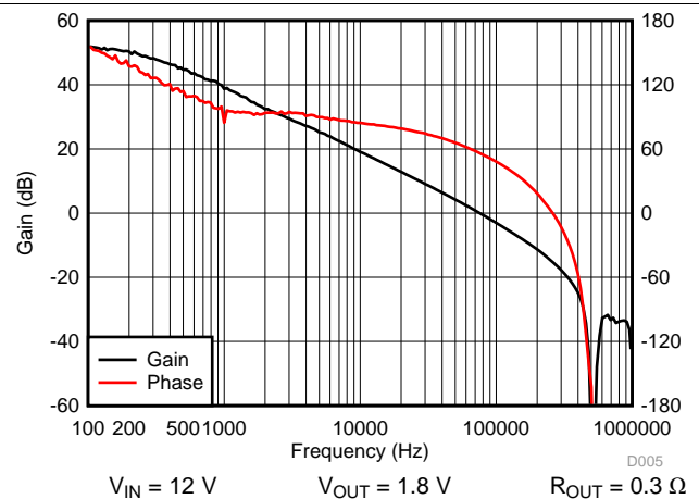
图 42. Loop Response
