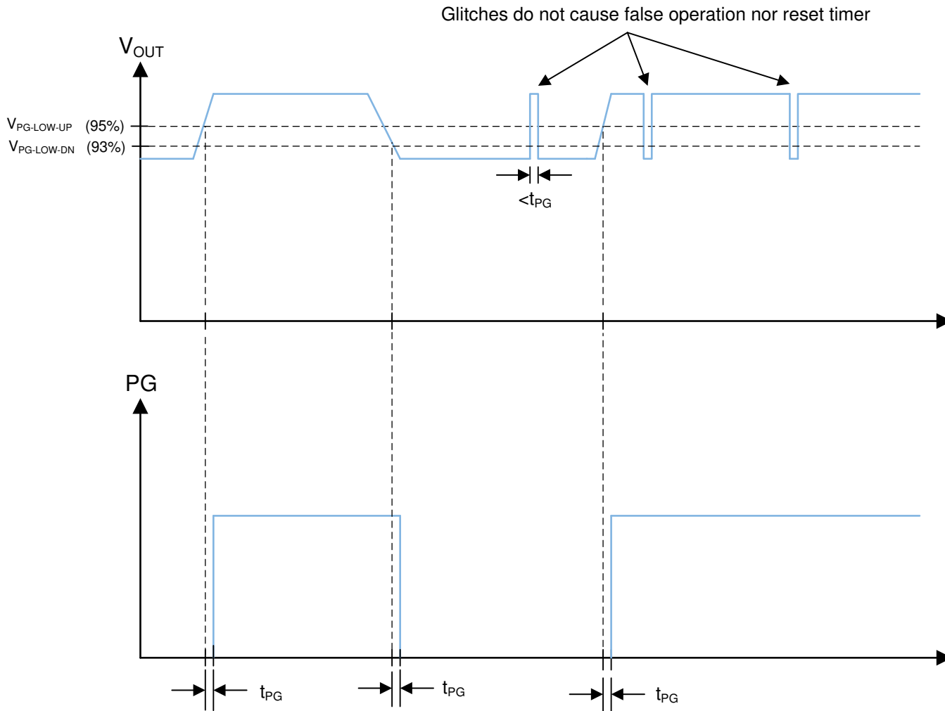
图 10. Power-Good-Timing Behavior
