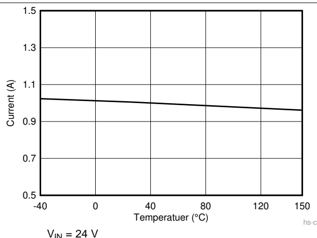
图 4. High Side Current Limit
