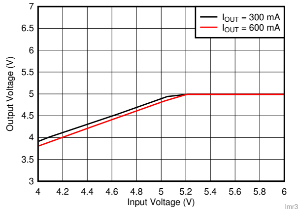
图 16. Overall Dropout Characteristic V_{OUT} = 5\text{ V}
