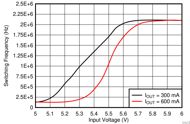
图 17. Typical f_{SW} vs Output Current f_{SW} = 2100\text{ kHz}
