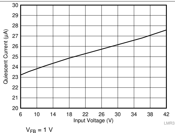
图 2. Non-Switching Input Supply Current
