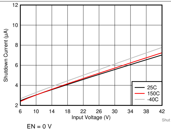
图 3. Shutdown Supply Current
