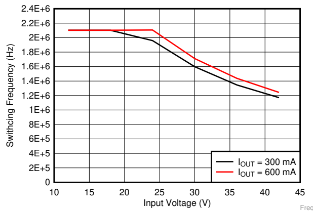
图 18. Switching Frequency vs Input Voltage V_{OUT} = 3.3\text{ V}
