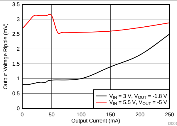
图 1. Output Voltage Ripple vs Output Current
