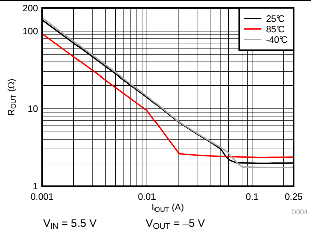
图 19. Charge-Pump Output Impedance vs Output Current
