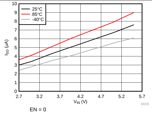
图 4. Shutdown Current
