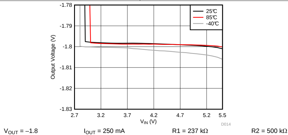
图 13. Line Regulation
