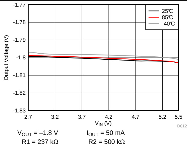
图 13. Line Regulation
