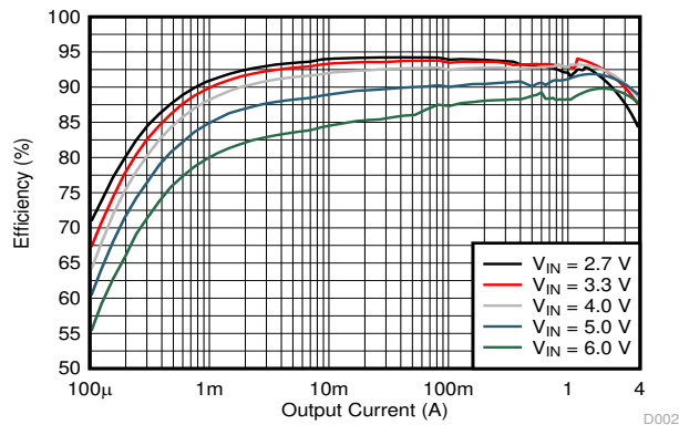
图 10-2. Efficiency versus Output Current
