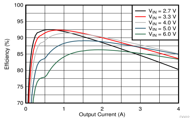
图 10-5. Efficiency versus Output Current
