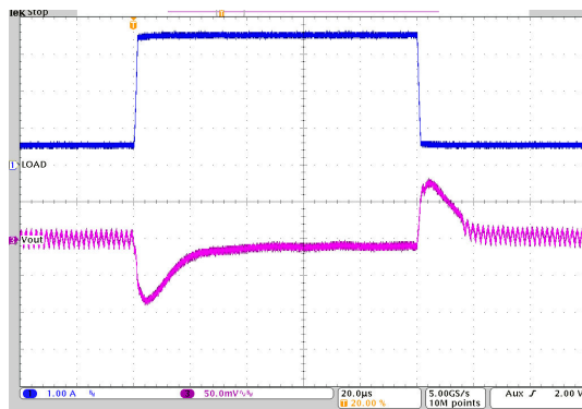
图 10-22. Load Transient Response
