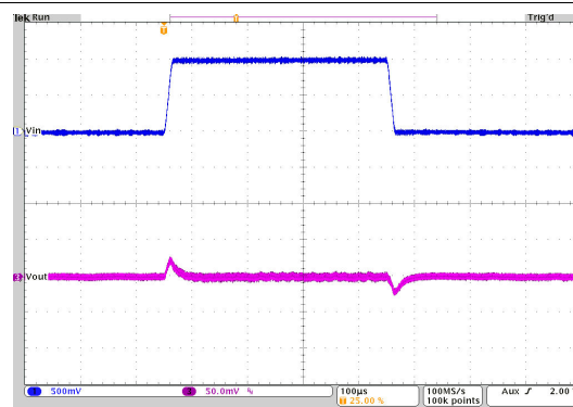
图 10-33. Line Transient Response
