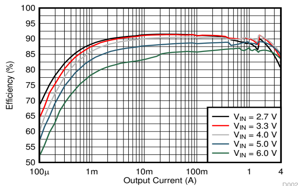
图 10-4. Efficiency versus Output Current
