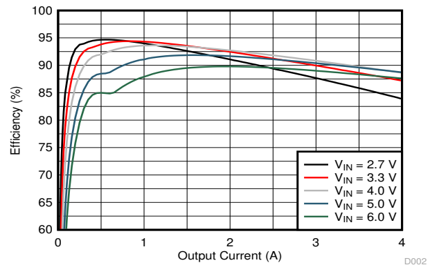
图 10-3. Efficiency versus Output Current
