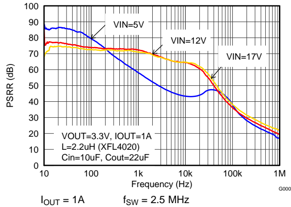
Figure 34. Power-Supply Rejection Ratio
