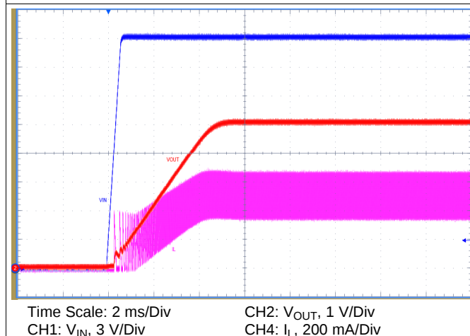
图 57. Full-Load Start-Up, V_{IN} = 24\text{ V}
