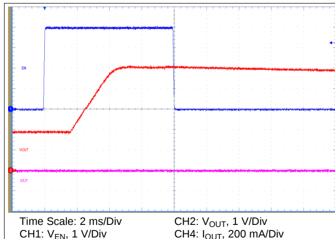
图 59. ENABLE On and Off; V_{OUT} Prebiased to 1.8 V V_{IN} = 24\text{ V} , No Load
