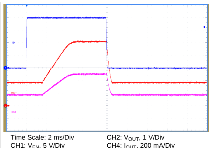
图 60. ENABLE On and Off; V_{OUT} Prebiased to 1.8 V V_{IN} = 24\text{ V} , 500 mA Load
