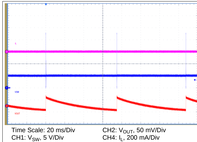
图 55. No-Load Switching Waveforms, V_{IN} = 24\text{ V}
