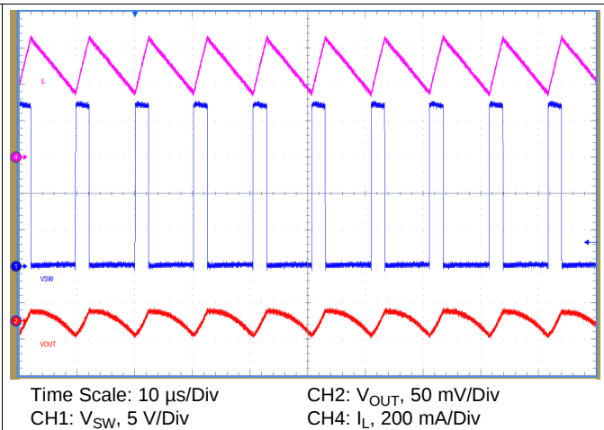
图 56. Full-Load Switching Waveforms, V_{IN} = 24\text{ V}
