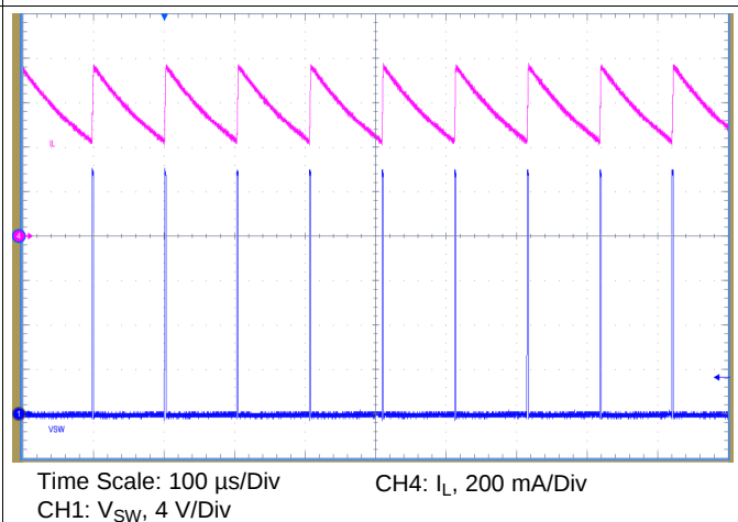
图 58. Short Circuit, V_{IN} = 24\text{ V}
