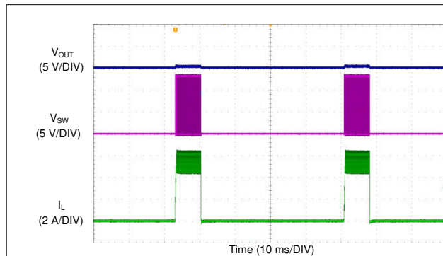
Figure 8-19. Inductor Current Bursts During Hiccup
