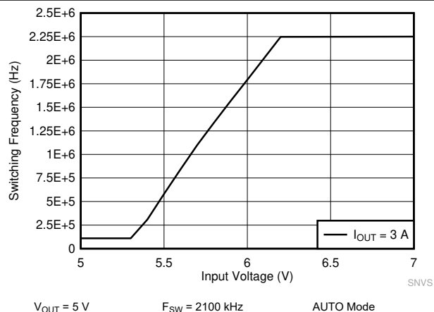
Figure 9-16. LM62435-Q1 Frequency Dropout Curve
