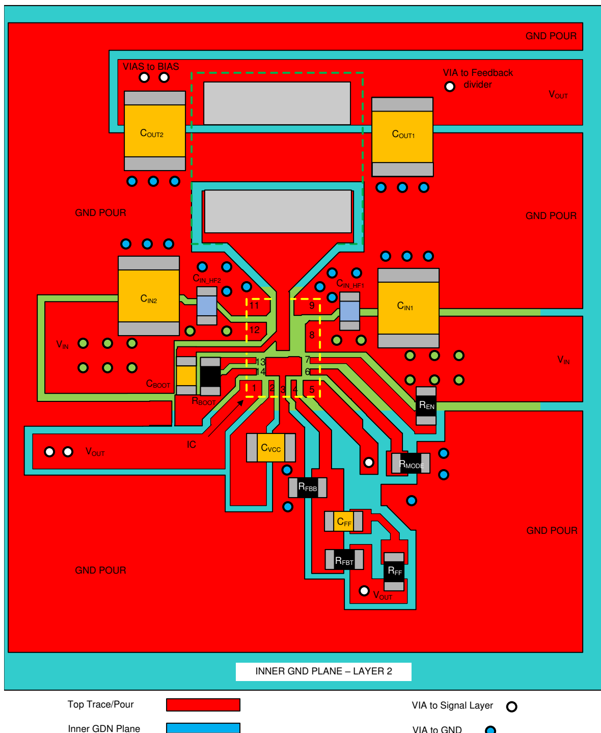
Figure 11-2. Layout Example
