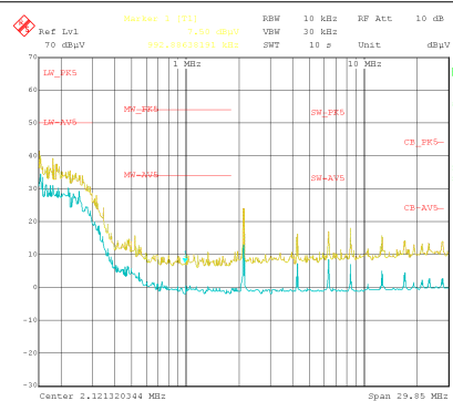
Figure 9-31. Radiated EMI Log Horizontal versus CISPR25 Limits
