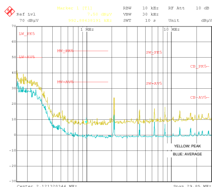
Conducted EMI: V_{OUT} = 5 \text{ V} , f_{SW} = 2100 \text{ kHz}
