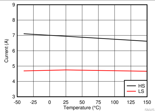
Figure 7-4. LM62435-Q1 High-side and Low-side Current Limits
