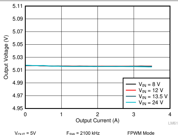
Figure 9-12. LM62435-Q1 Load and Line Regulation
