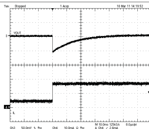
Figure 42. 负载瞬态
