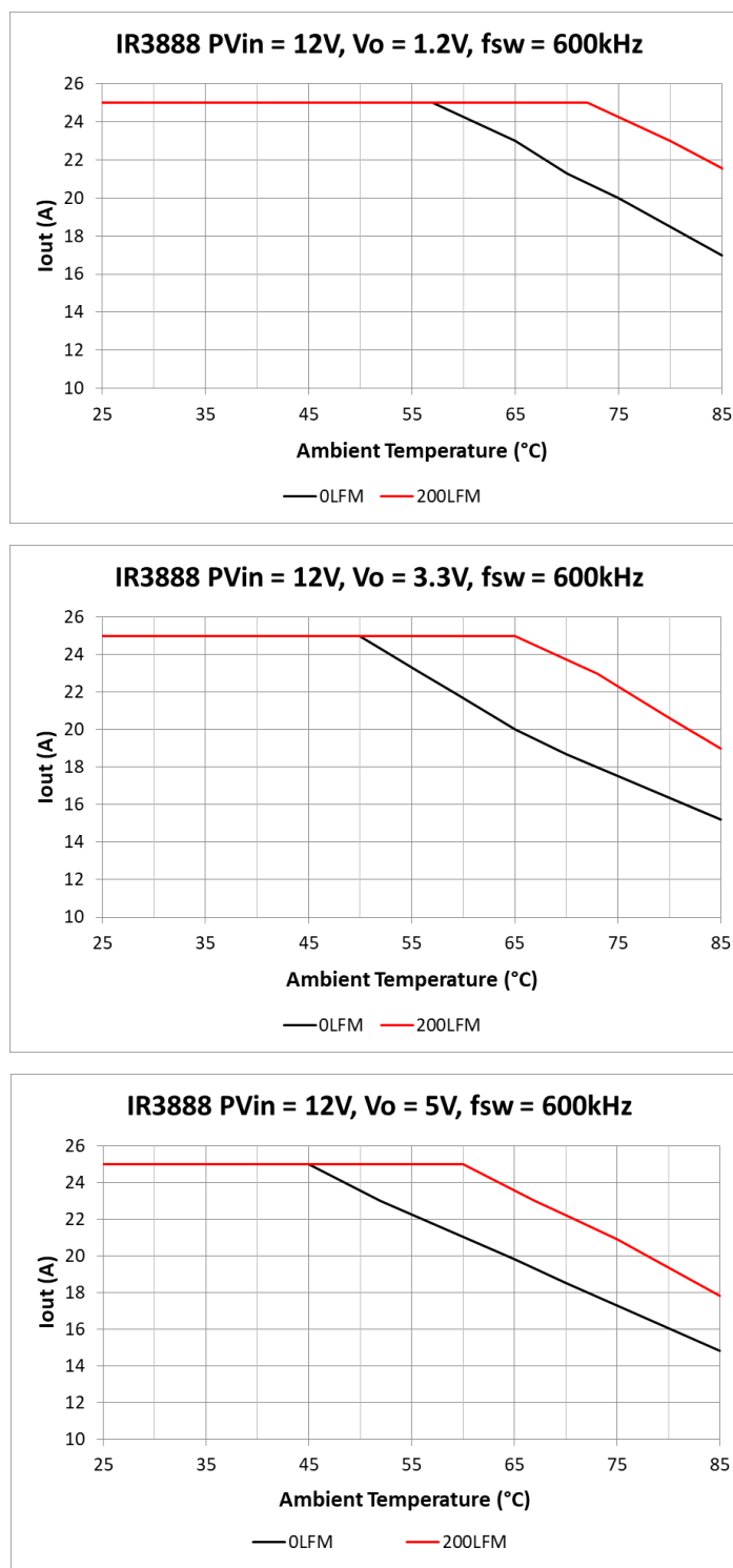
Figure 4 Thermal de-rating curves, PV_{in} = 12\text{ V} , V_{out}=1.0\text{ V}/3.3\text{ V}/5\text{ V} , f_{sw} = 600\text{ kHz} , VCC = Internal LDO
