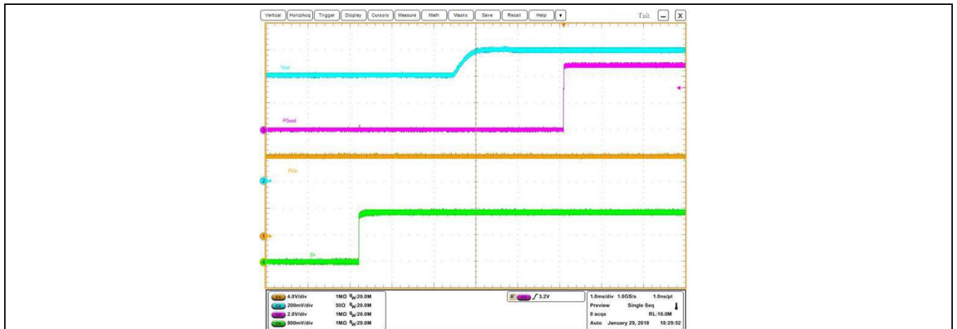
Figure 17 Pre-bias Start up at 0 A Load, (Ch 1 : PVin, Ch 2 : Vo, Ch 3 : PGGood, Ch 4 : En)
