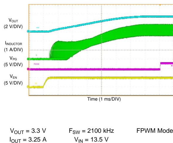
图 56. LM61440 Start-up with 3.25-A
