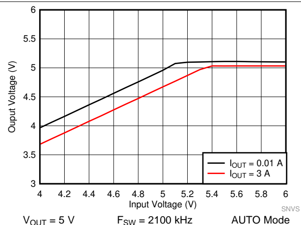
图 49. LM61440 Dropout Curve
