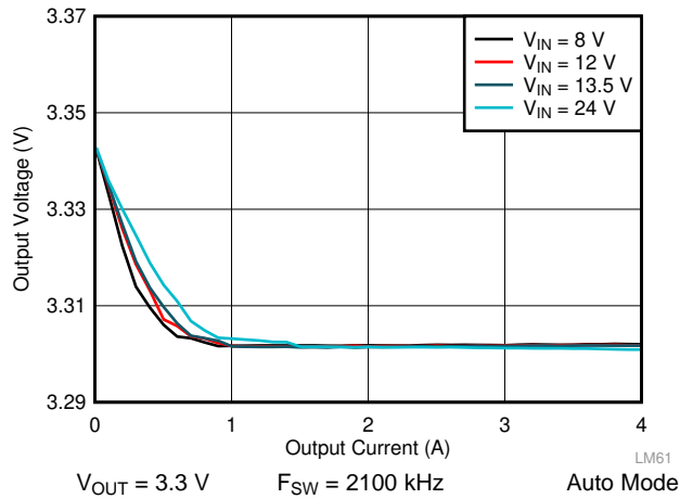
图 40. LM61440 Load and Line Regulation
