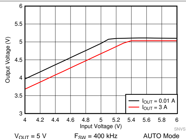
图 48. LM61440 Dropout Curve
