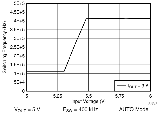
图 52. LM61440 Frequency Dropout Curve
