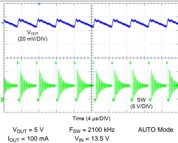
图 54. LM61440 Switching Waveform and VOUT Ripple
