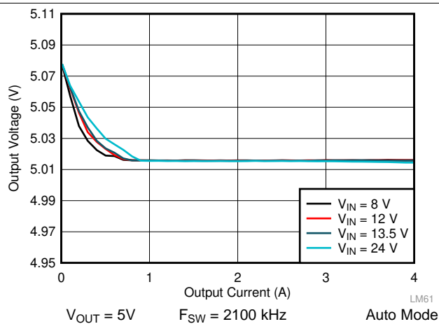
图 44. LM61440 Load and Line Regulation
