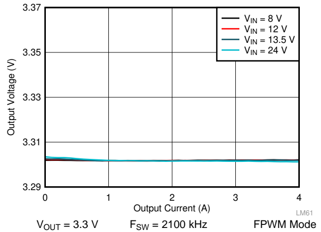
图 41. LM61440 Load and Line Regulation
