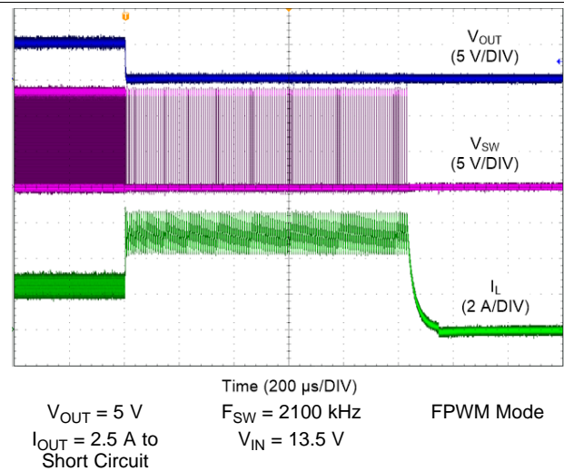
图 57. LM61440 Short Circuit Protection
