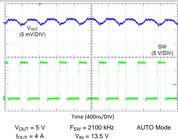
图 55. LM61440 Switching Waveform and VOUT Ripple
