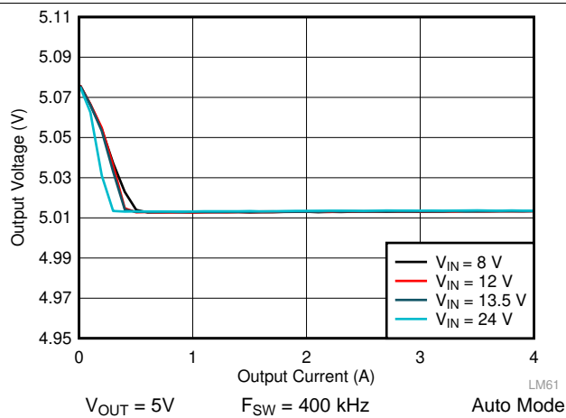
图 42. LM61440 Load and Line Regulation
