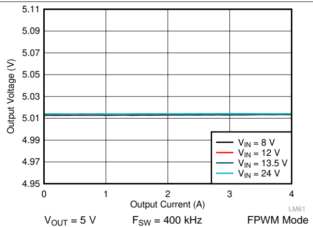
图 43. LM61440 Load and Line Regulation
