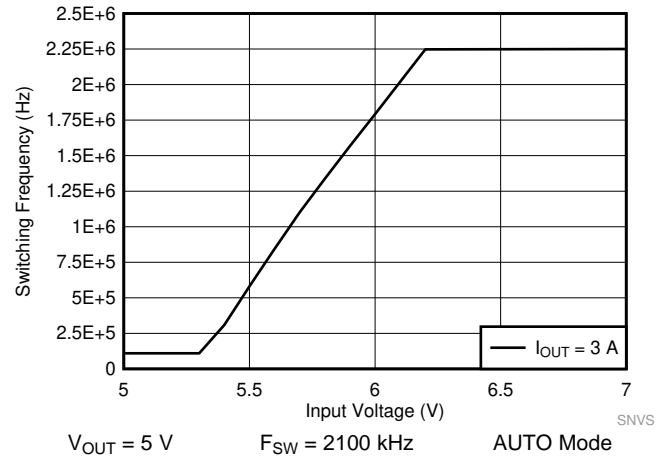
图 53. LM61440 Frequency Dropout Curve
