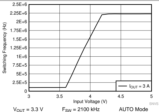
图 51. LM61440 Frequency Dropout Curve
