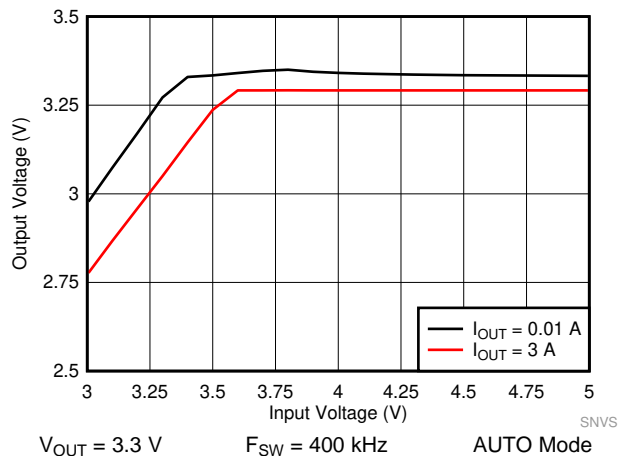
图 46. LM61440 Dropout Curve
