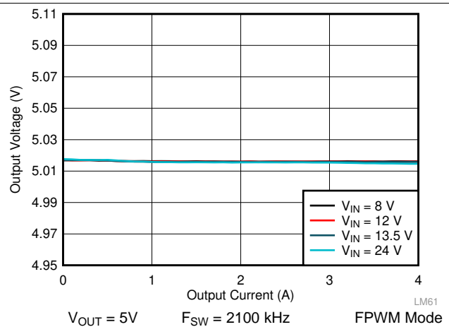
图 45. LM61440 Load and Line Regulation
