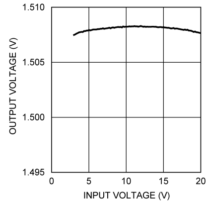
Figure 8. Line Regulation - L1 = 4.7\text{ }\mu\text{H} V_{OUT} = 1.5\text{ V} , I_{OUT} = 500\text{ mA}
