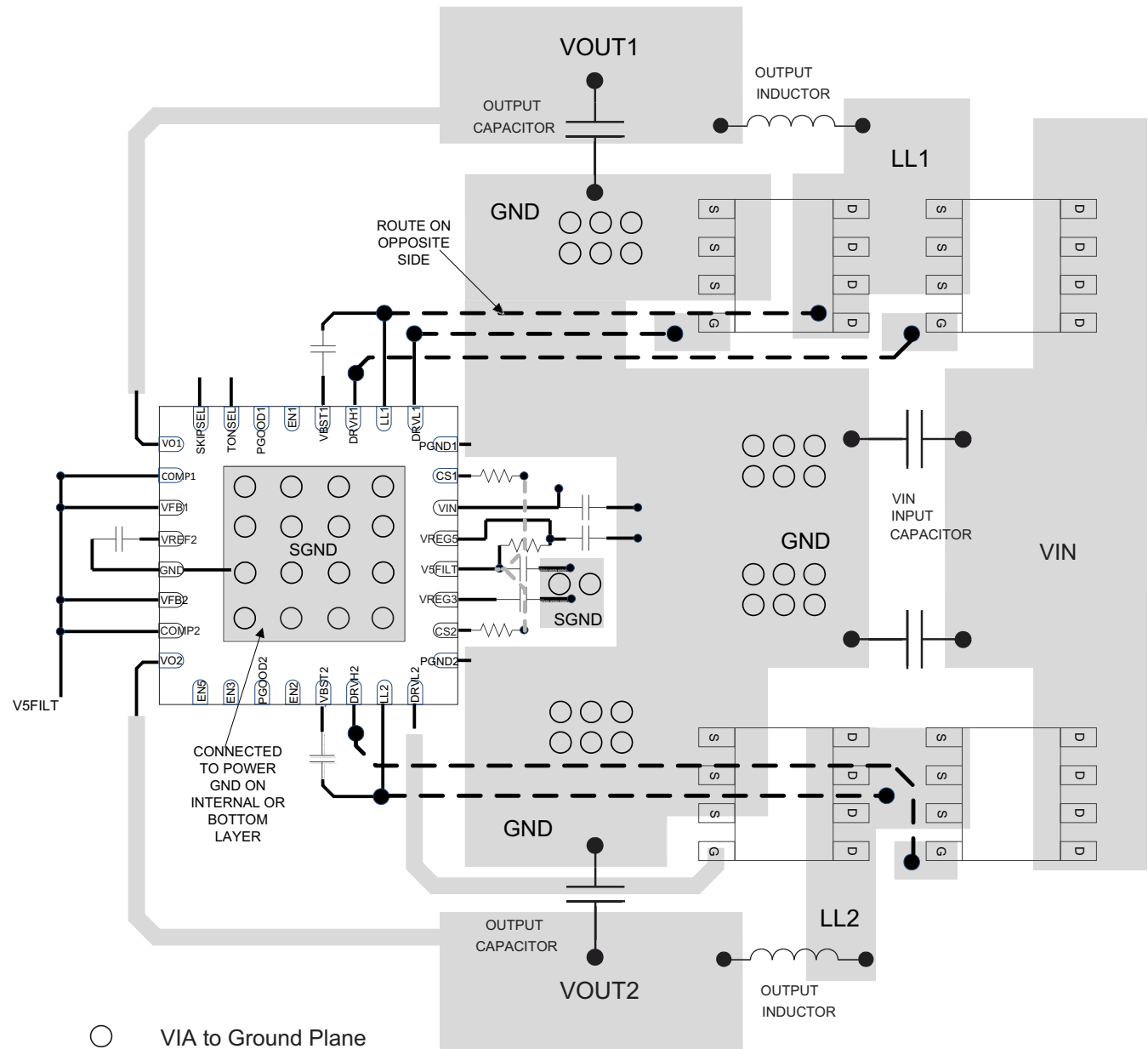
Figure 41. Layout Example
