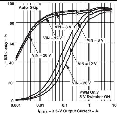
Figure 26. 3.3-V Efficiency vs Output Current
