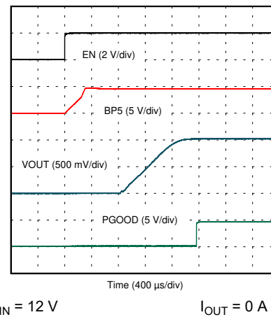
Figure 8-9. EN Start-up – Measuring BP5
