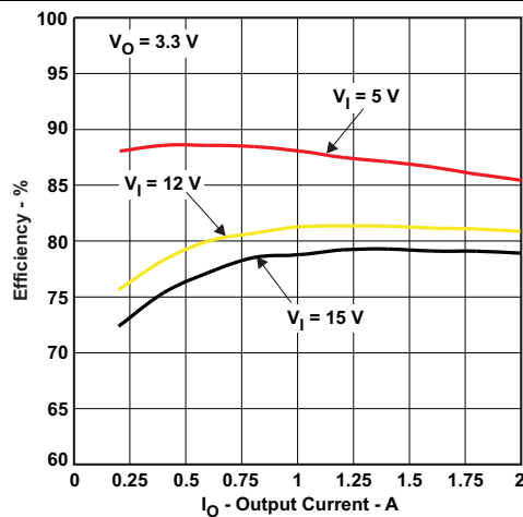
Figure 13. TPS54232 Efficiency
