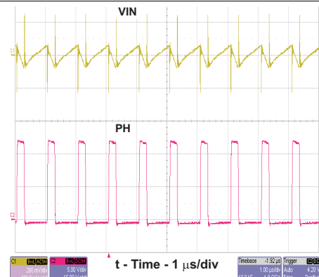
Figure 20. TPS54232 Input Ripple
