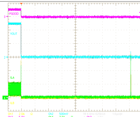
图 34. Shutdown Through VIN
