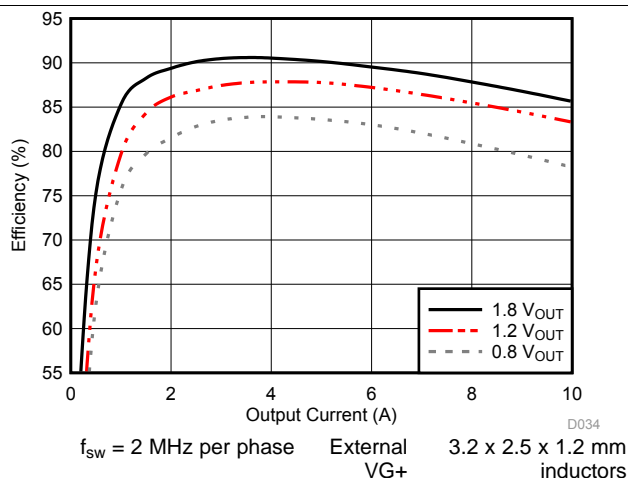
图 20. Efficiency vs Output Current for Output Voltage
