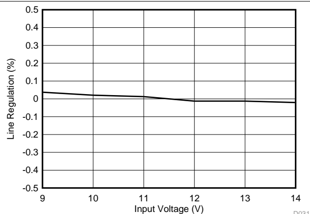
图 51. Line Regulation
