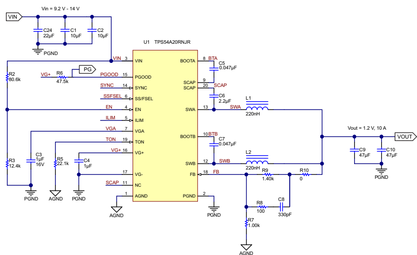
图 47. Typical Application
