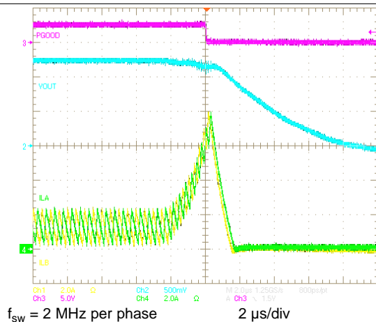
图 35. Short Circuit Protection
