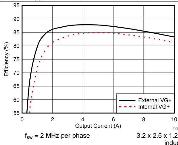
图 19. Efficiency vs Output Current for Gate Drive Supply
