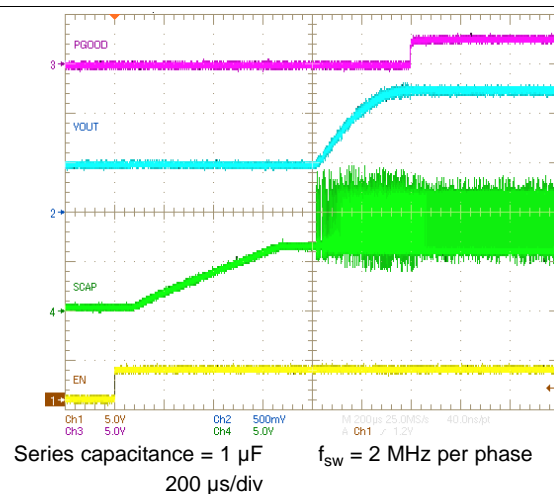
图 30. Pre-biased Startup Through EN
