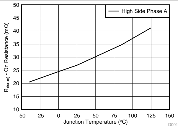
图 1. On Resistance vs Junction Temperature
