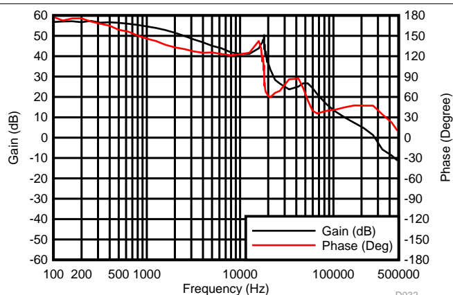
图 52. Loop Response
