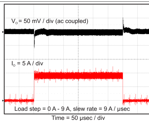
图 53. Transient Response
