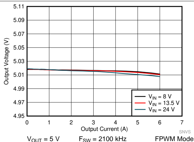
图 50. LM61460-Q1 Load and Line Regulation
