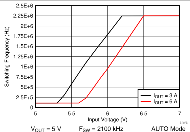
图 58. LM61460-Q1 Frequency Dropout Curve
