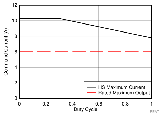
图 20. Maximum Current Allowed Through the HS FET - Function of Duty Cycle for LM61460-Q1
