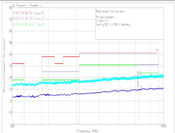
图 80. Radiated EMI Bicon Horizontal versus CISPR25 Limits
