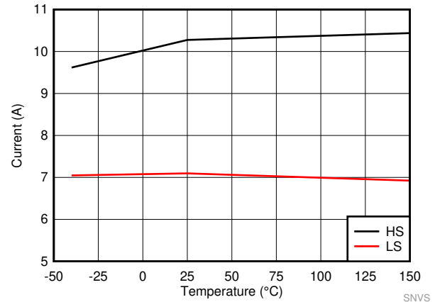
图 4. LM61460-Q1 High-side and Low-side Current Limits
