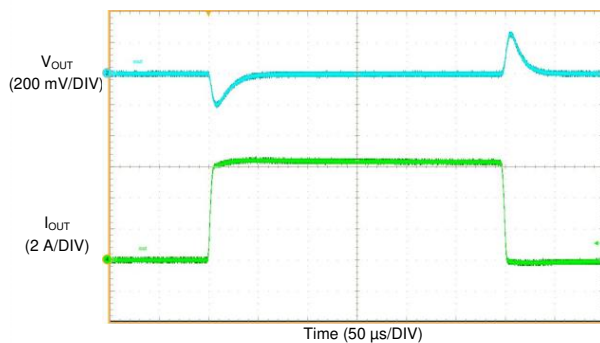
图 67. Graceful Recovery from Dropout
