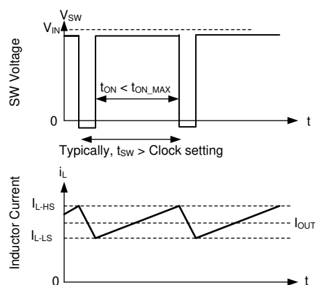
图 21. Current Limit Waveforms
