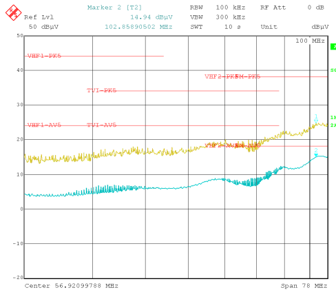
图 77. Conducted EMI versus CISPR25 Limits (Yellow: Peak Signal, Blue: Average Signal)
