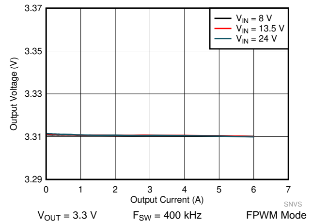
图 44. LM61460-Q1 Load and Line Regulation
