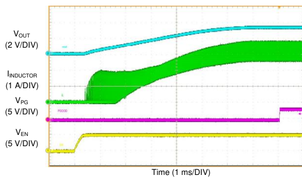
图 61. LM61460-Q1 Start-up with 50-mA Load
