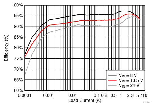
效率: V_{OUT} = 5V , F_{SW} = 400\text{kHz}
