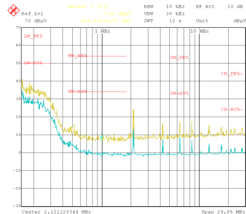
图 84. Conducted EMI versus CISPR25 Limits (Yellow: Peak Signal, Blue: Average Signal)
