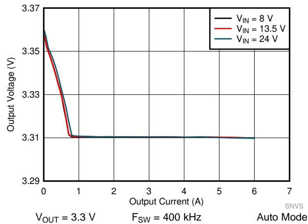
图 43. LM61460-Q1 Load and Line Regulation
