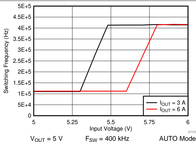
图 57. LM61460-Q1 Frequency Dropout Curve
