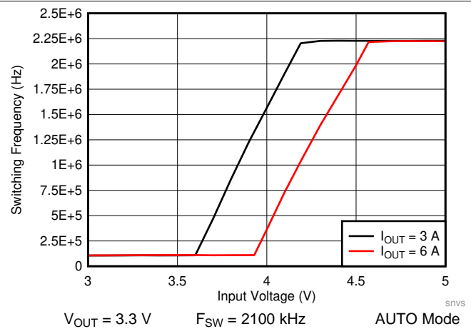
图 56. LM61460-Q1 Frequency Dropout Curve
