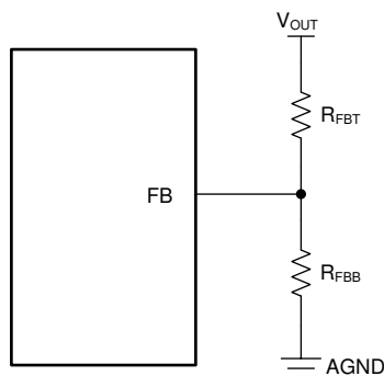
图 19. Setting Output Voltage of Adjustable Versions
