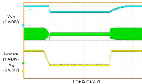
图 18. Recovery From Dropout ( V_{OUT} = 5\text{ V} , I_{OUT} = 4\text{ A} , V_{IN} = 13.5\text{ V} to 4\text{ V} to 13.5\text{ V} )
