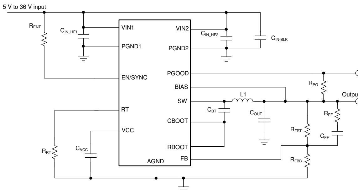
图 31. Example Application Circuit
