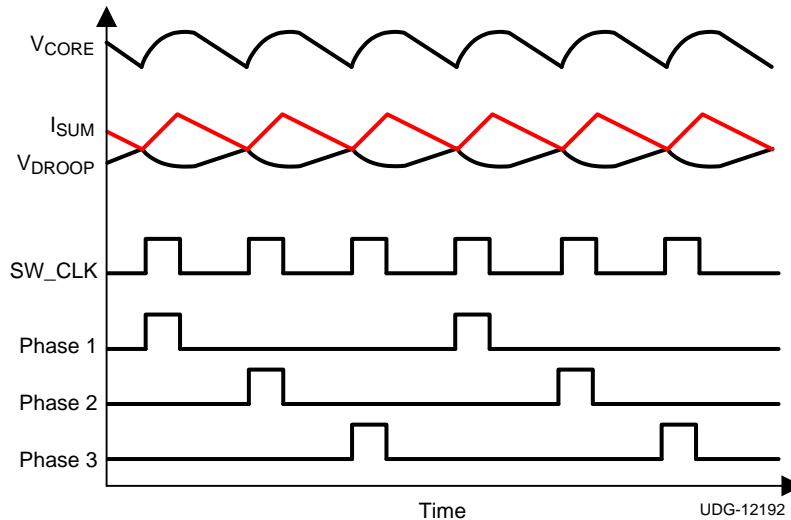
图 21. D-CAP+™ Mode Basic Waveforms
