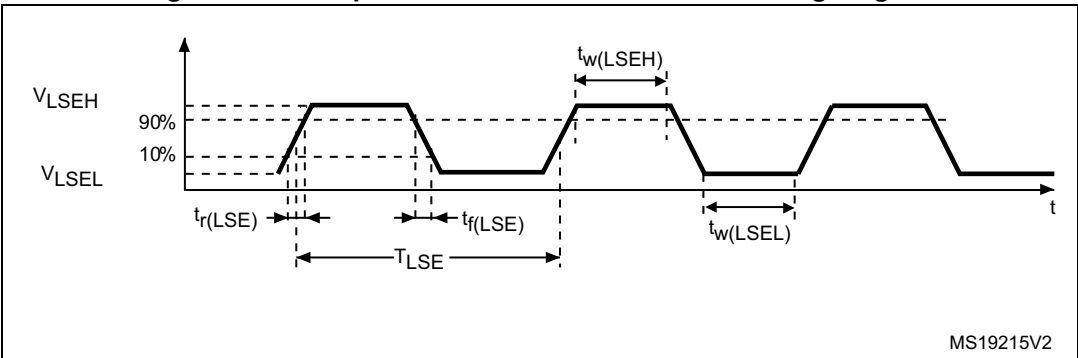
Figure 16. Low-speed external clock source AC timing diagram
