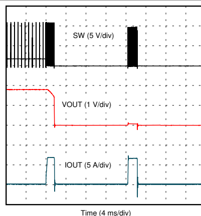
图 8-29. Overcurrent Response
