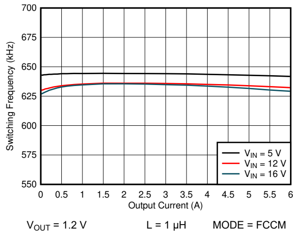
图 6-15. 600-kHz Switching Frequency vs Load Current
