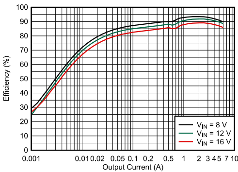
图 8-4. Efficiency - 1100 kHz, FCCM, External 3.3-V VCC, 4.7- \Omega R_{BOOT}
