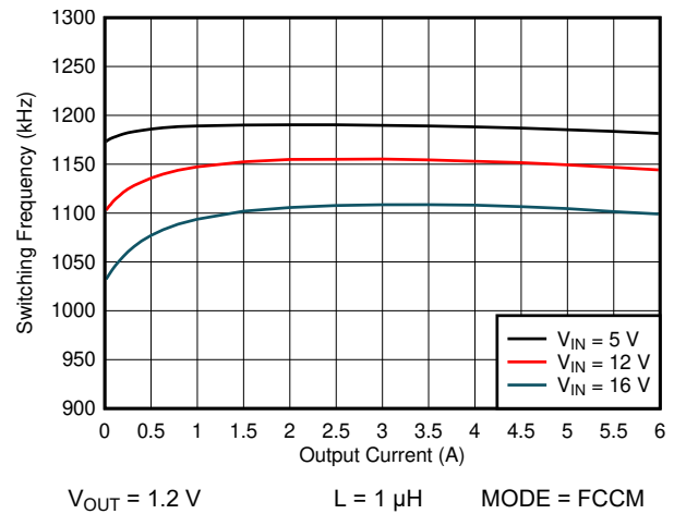
图 6-16. 1100 kHz Switching Frequency vs Load Current
