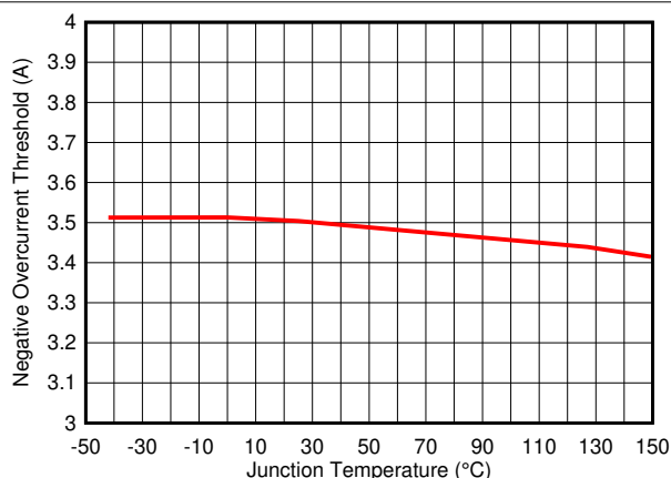
图 6-4. Negative Overcurrent Limit
