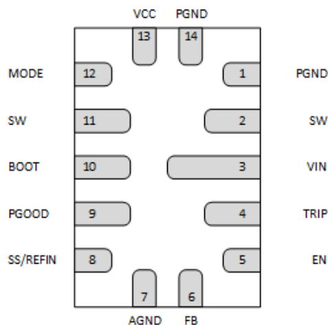
图 5-2. 14-Pin QFN RPG Package (Bottom View)
