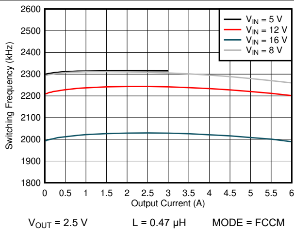
图 6-17. 2200 kHz Switching Frequency vs Load Current
