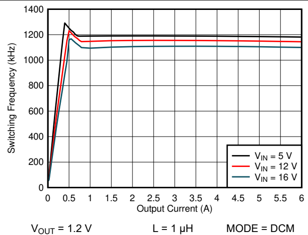
图 6-18. 1100 kHz Switching Frequency vs Load Current - DCM
