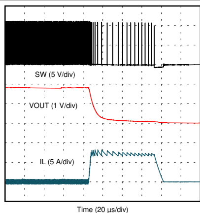
图 8-28. Overcurrent Response
