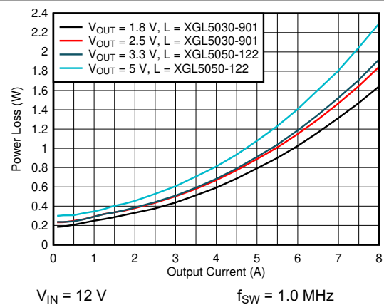
图 6-6. Power Loss vs Output Current - 1.8-V to 5.0-V Output
