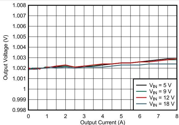
图 8-5. Load Regulation
