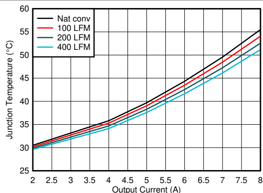
图 6-7. Junction Temperature vs Output Current - 1-V Output
