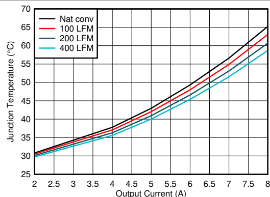
图 6-8. Junction Temperature vs Output Current - 3.3-V Output
