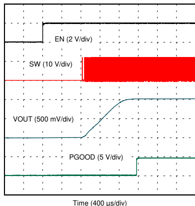
V_{IN} = 12\text{ V} I_{OUT} = 0\text{ A} 图 8-10. EN Startup - Measuring SW
