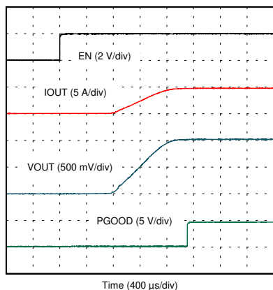
V_{IN} = 12\text{ V} R_{OUT} = 0.2\ \Omega 图 8-12. EN Start-up - With Load
