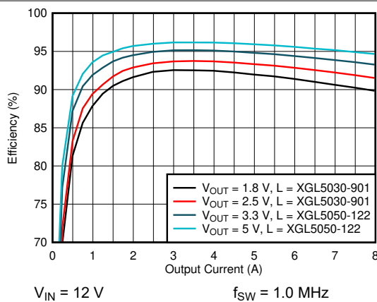
图 6-5. Efficiency vs Output Current - 1.8-V to 5.0-V Output
