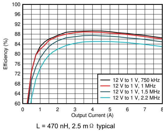
图 6-1. Efficiency vs Output Current
