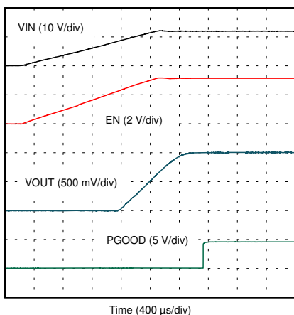
R_{OUT} = 0.3\ \Omega 图 8-14. VIN Start-up
