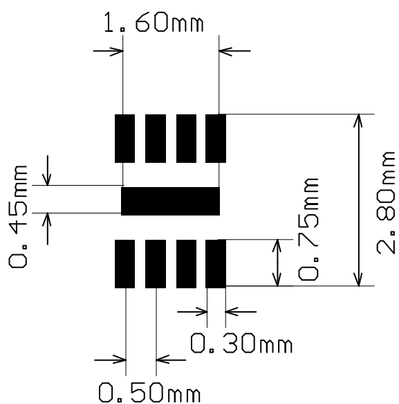
Figure 53. DFN8 2x2 recommended footprint
