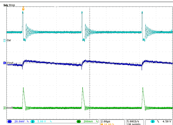
Figure 36. Typical Operation in Power Save Mode ( I_{OUT}=10\text{ mA} )
