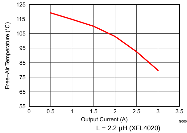
Figure 43. Maximum Ambient Temperature
