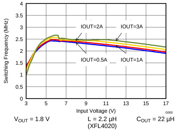
Figure 31. Switching Frequency vs. Input Voltage
