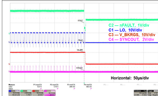
Figure 65. nFAULT Shutdown Latch
