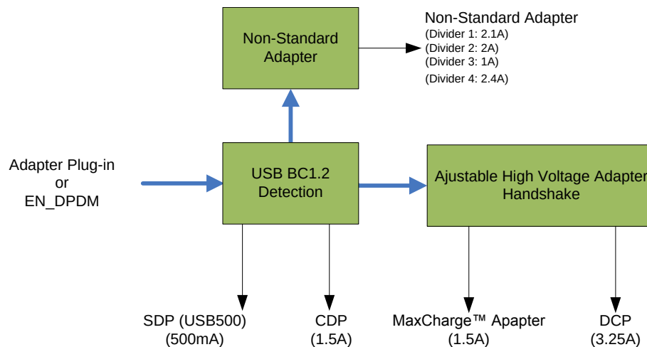
图 9. USB D+/D- Detection
