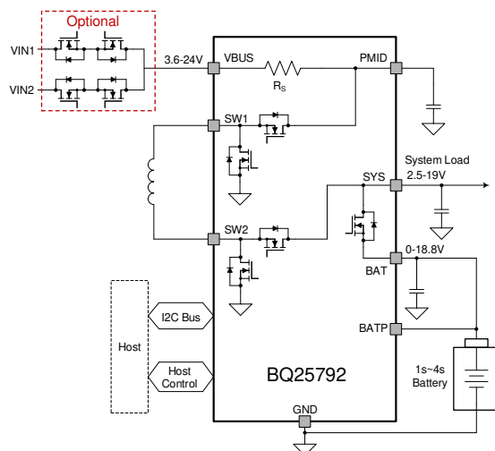
Simplified Schematic
