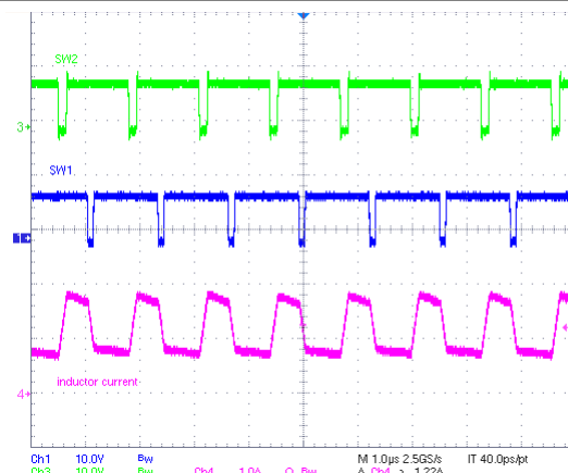
Figure 10-8. Buck-Boost Charging Mode PWM Operation
