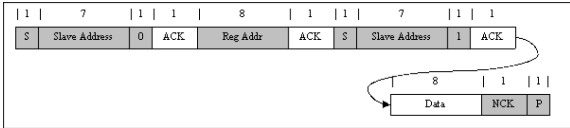
Figure 9-21. Single Read
