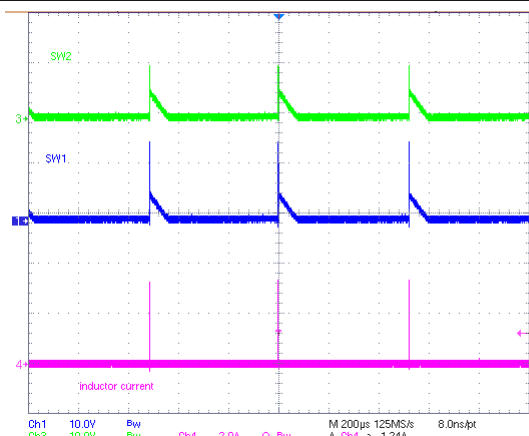
Figure 10-9. Buck Charging Mode PWM Operation
