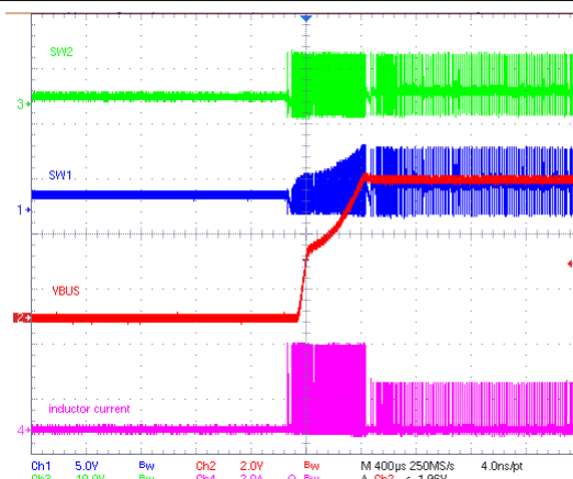
Figure 10-10. Buck Mode PFM with OOA
