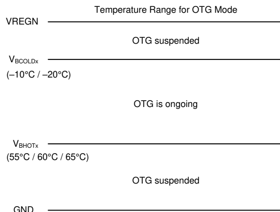
Figure 9-12. TS Pin Thermistor Sense Threshold in OTG Mode
