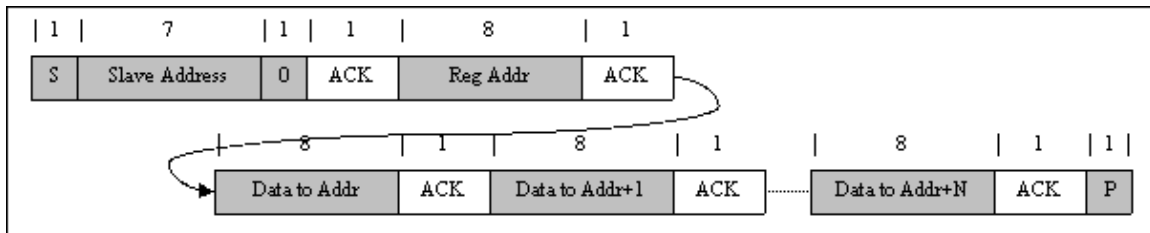
Figure 9-22. Multi-Write
