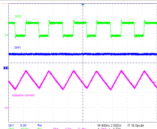
Figure 10-7. Boost Charging Mode PWM Operation
