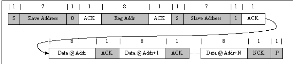
Figure 9-23. Multi-Read
