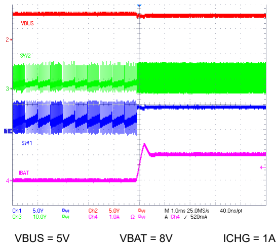
Figure 10-5. Charge Enable
