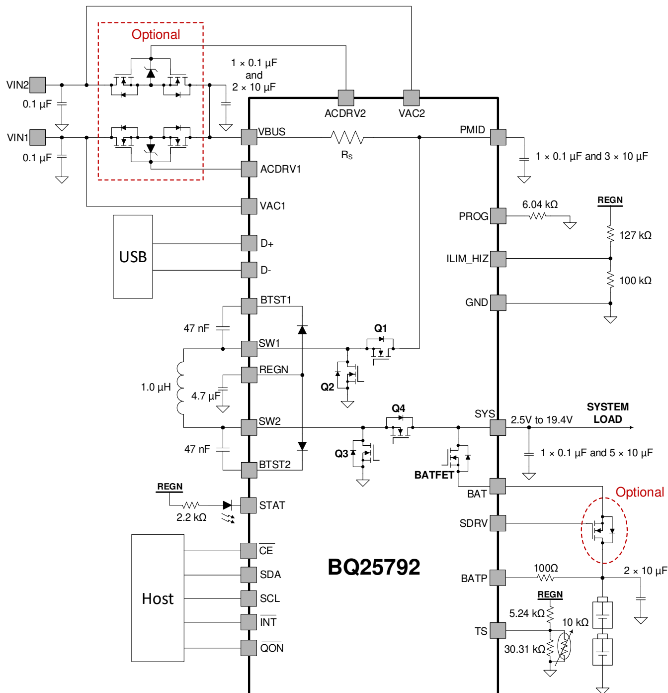
Figure 10-1. BQ25792 Application Diagram with Two Input Sources and Ship FET
