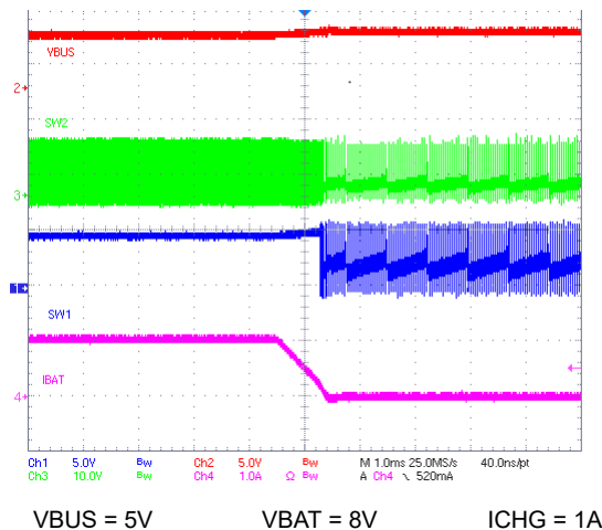
Figure 10-6. Charge Disable
