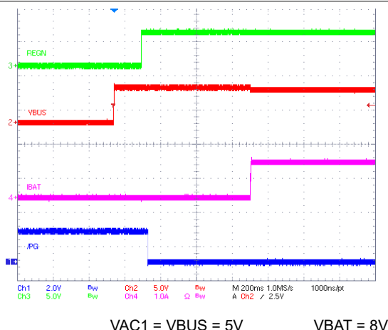
Figure 10-4. Power Up from VAC1 with Charge Enabled
