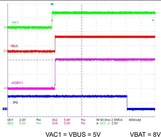
Figure 10-3. ACFET1-RBFET1 Turns on at Power Up
