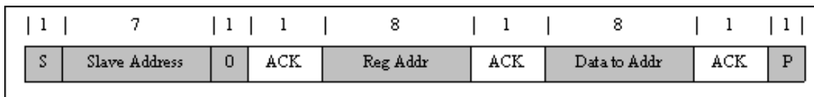
Figure 9-20. Single Write
