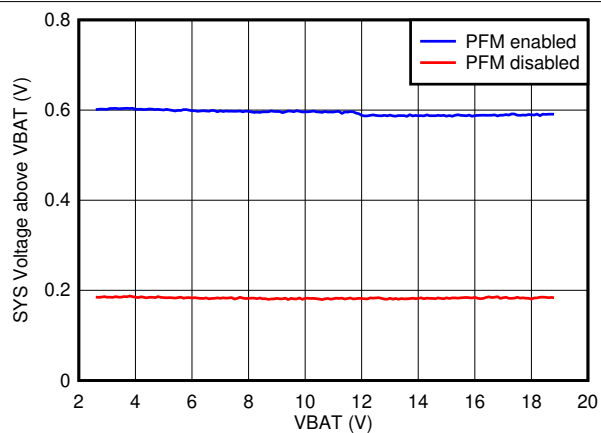
Figure 7-20. Offset Voltage of SYS Regulation above VBAT
