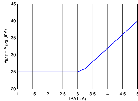
Figure 8-8. BATFET I-V Curve
