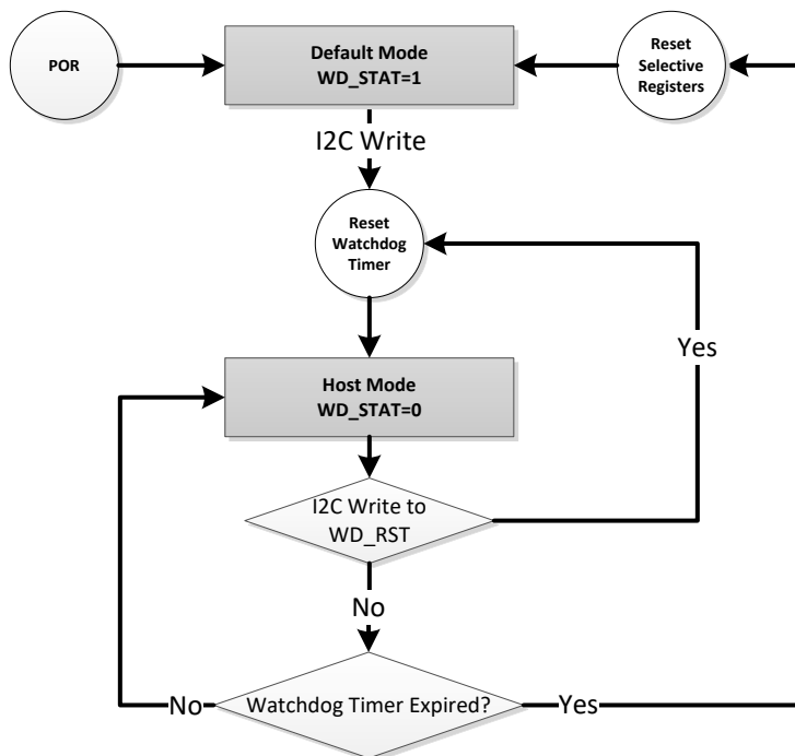
Figure 8-25. Watchdog Timer Flow Chart
