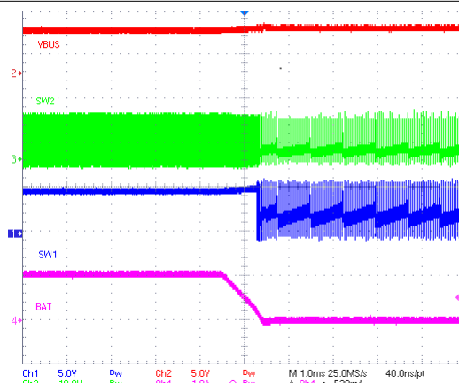
Figure 9-5. Power Up from VAC1 with Charge Enabled
