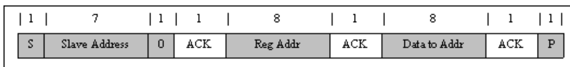
Figure 8-21. Single Write
