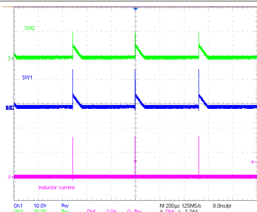
Figure 9-10. Buck Charging Mode PWM Operation
