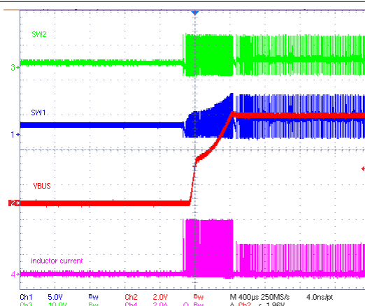
Figure 9-11. Buck Mode PFM with OOA
