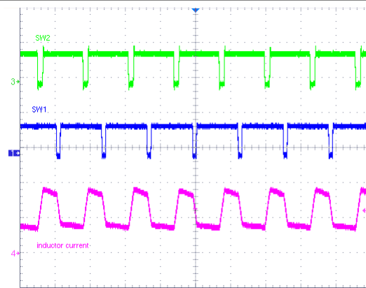
Figure 9-9. Buck-Boost Charging Mode PWM Operation
