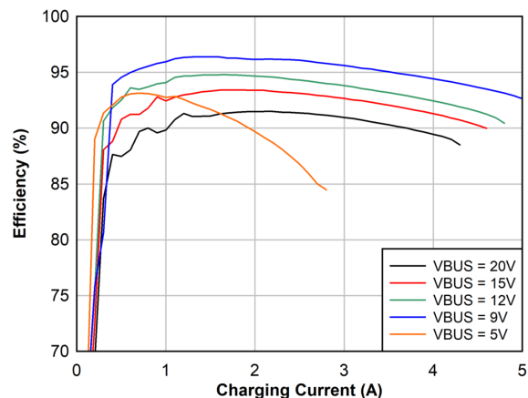
Figure 7-4. 2s Battery Charge Efficiency, 1.5 MHz
