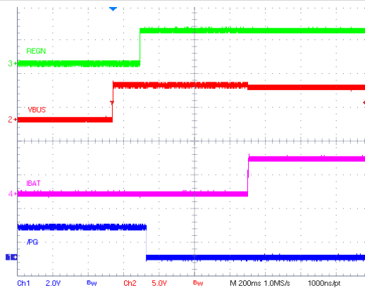
Figure 9-5. Power Up from VAC1 with Charge Enabled
