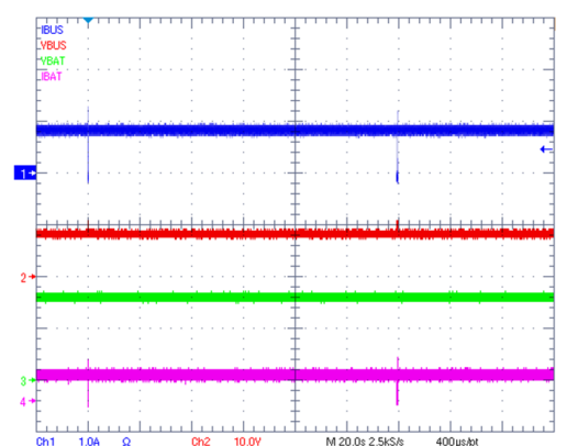
Figure 9-16. IINDPM Transient Response
