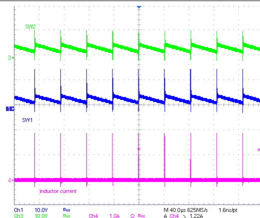
Figure 9-9. Buck-Boost Charging Mode PWM Operation
