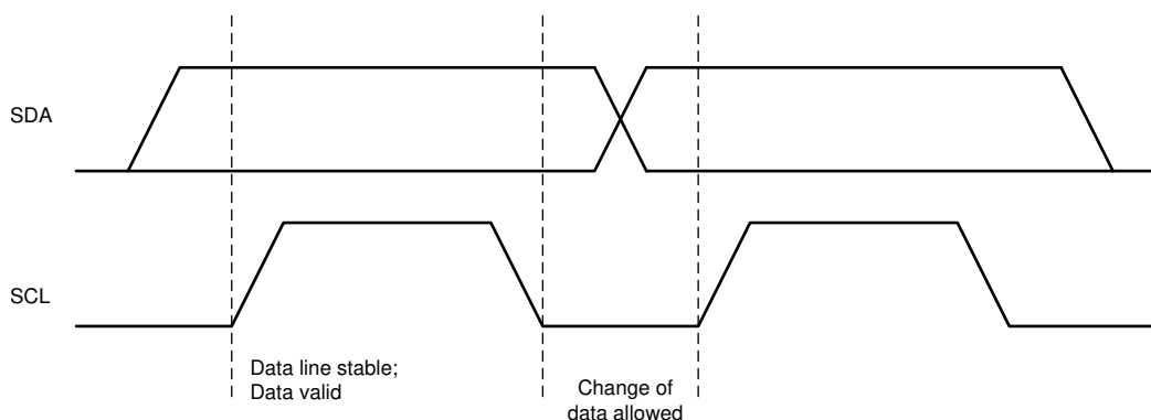
Figure 8-16. Bit Transfers on the I 2 C Bus
