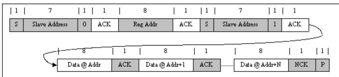
Figure 8-24. Multi-Read
