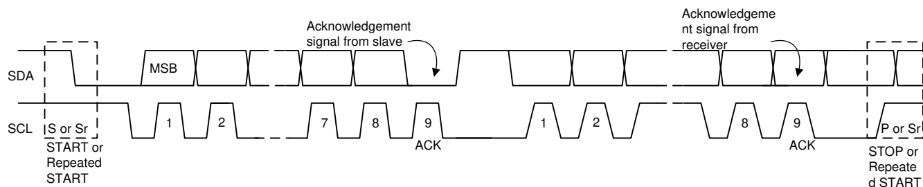
Figure 8-18. Data Transfer on the I²C Bus
