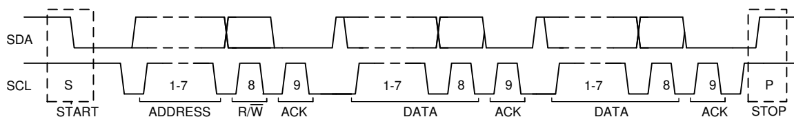
Figure 8-20. Complete Data Transfer on the I²C Bus
