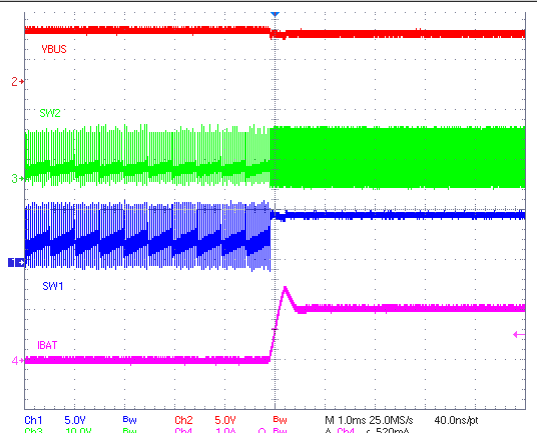
Figure 9-6. Charge Enable
