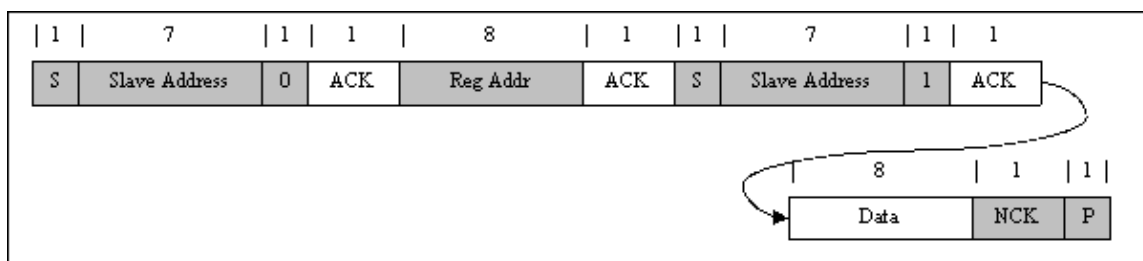
Figure 8-22. Single Read
