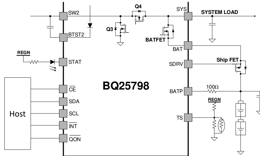
Figure 8-15. The Application Diagram for the External Ship FET
