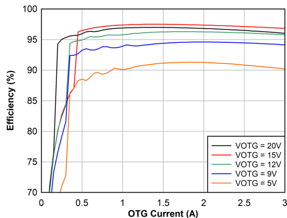
Figure 7-15. 4s Battery OTG Efficiency, 750 kHz
