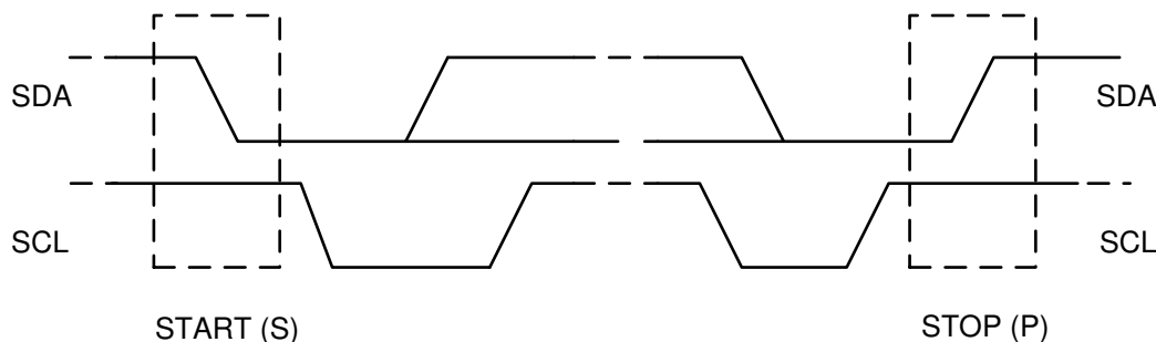
Figure 8-17. START and STOP Conditions on the I 2 C Bus
