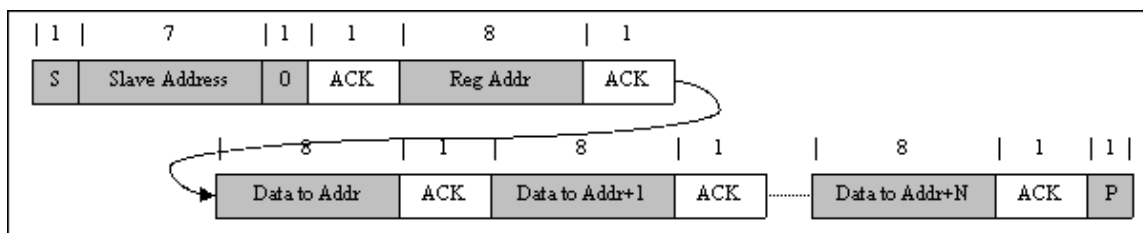
Figure 8-23. Multi-Write
