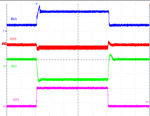
Figure 9-14. OTG Startup at 500-mA Load
