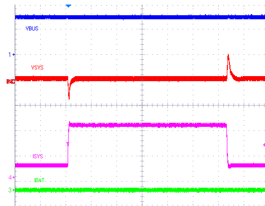
Figure 9-15. VSYS Load Transient Response
