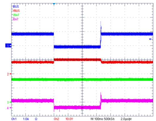
Figure 9-17. VOTG Load Transient Response
