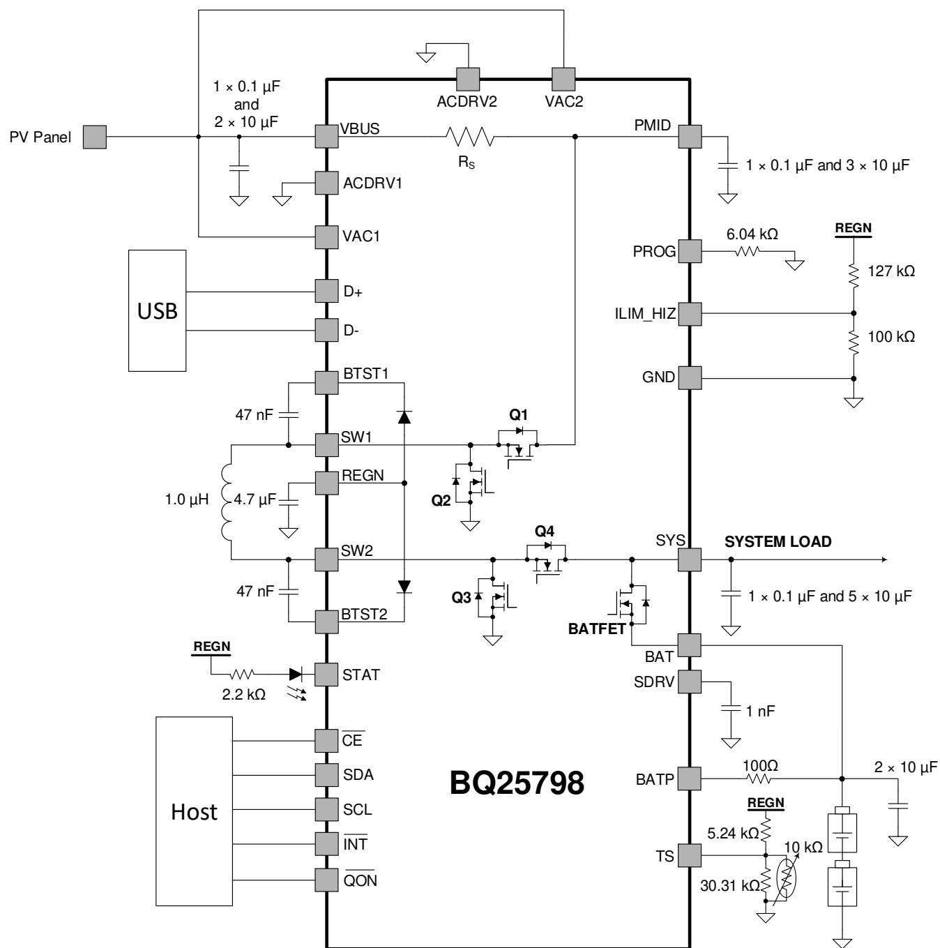
Figure 9-1. BQ25798 Application Diagram with Single Input Source and No Ship FET
