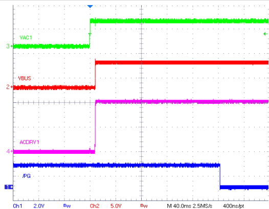
Figure 9-4. ACFET1-RBFET1 Turns on at Power Up
