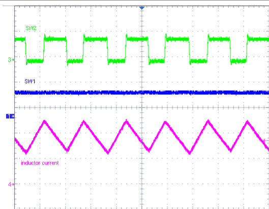
Figure 9-8. Boost Charging Mode PWM Operation
