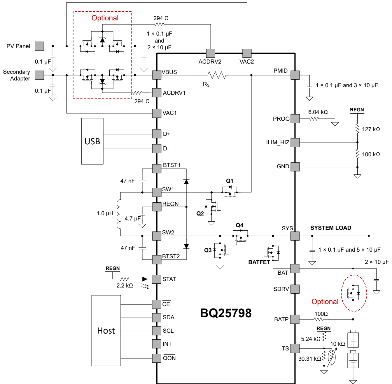
Figure 9-2. BQ25798 Application Diagram with Two Input Sources and Ship FET
