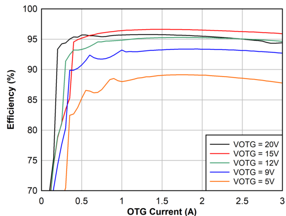
Figure 7-16. 4s Battery OTG Efficiency, 1.5 MHz
