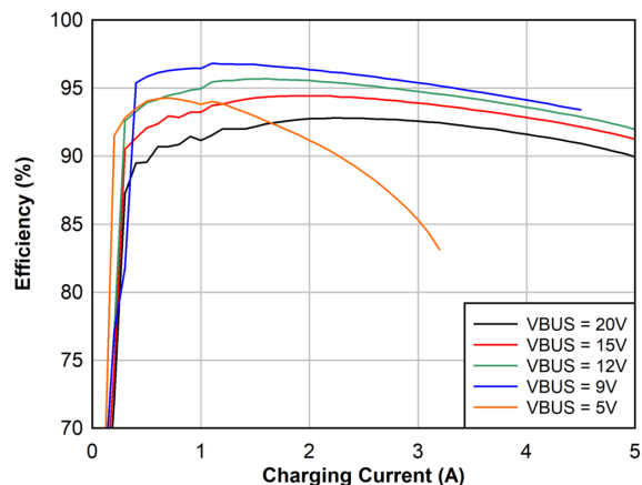
Figure 7-3. 2s Battery Charge Efficiency, 750 kHz
