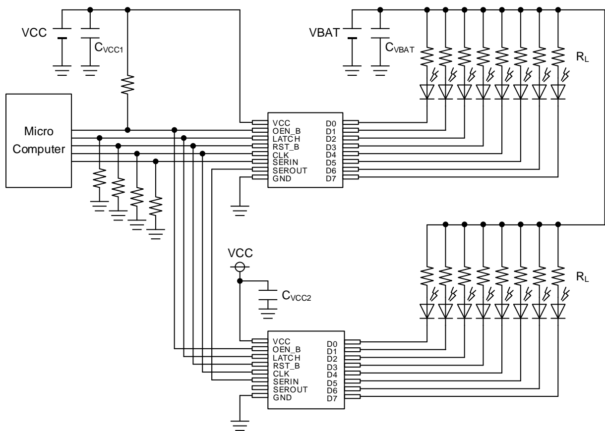
Figure 19. Application Example
