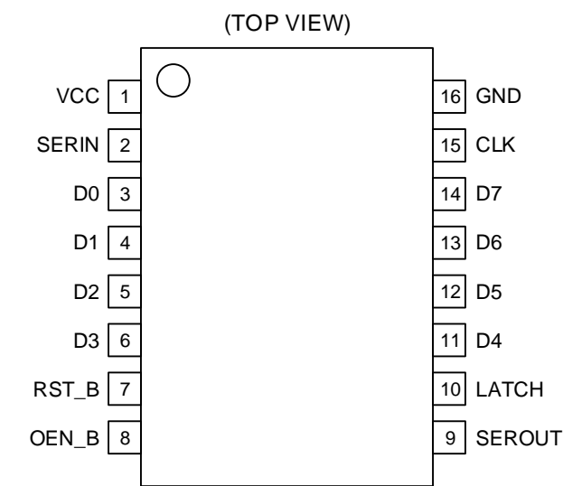
Figure 2. Pin Configuration
