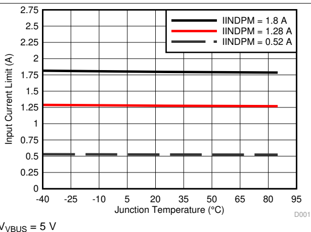
Figure 4. Input Current Limit vs. Junction Temperature
