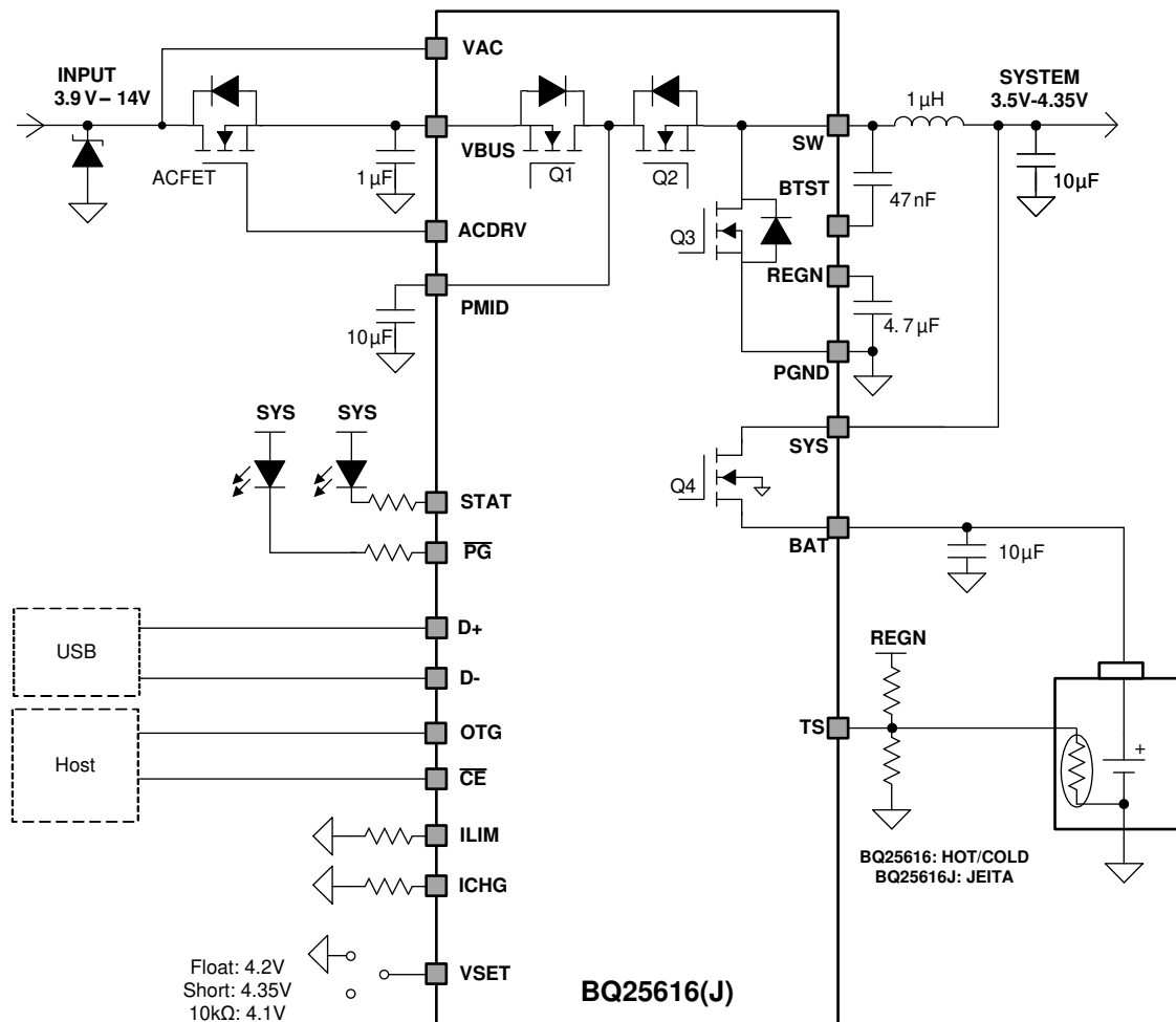
Figure 36. BQ25616/616J Application Diagram with External OVP
