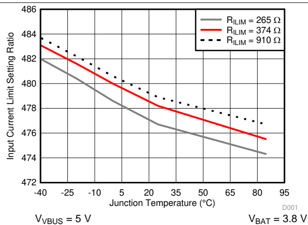
Figure 6. Input Current Limit Setting Ratio vs. Junction Temperature
