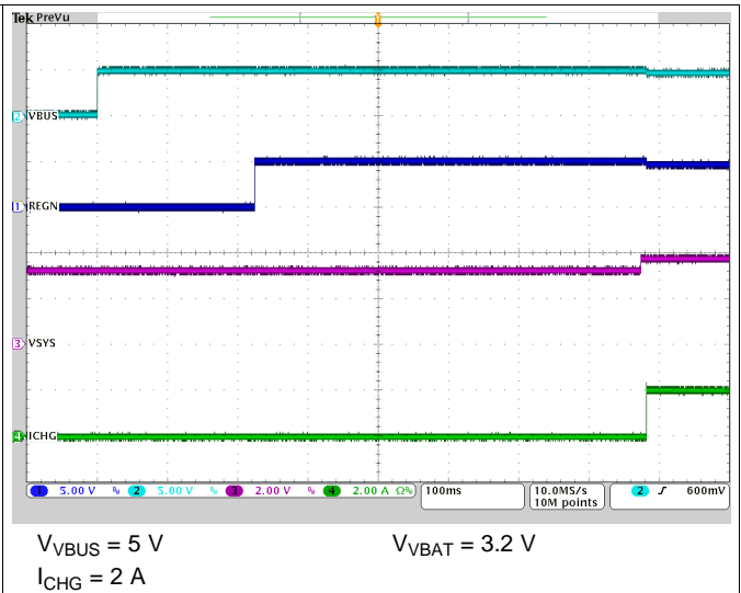
Figure 17. Power-Up with Charge Enabled
