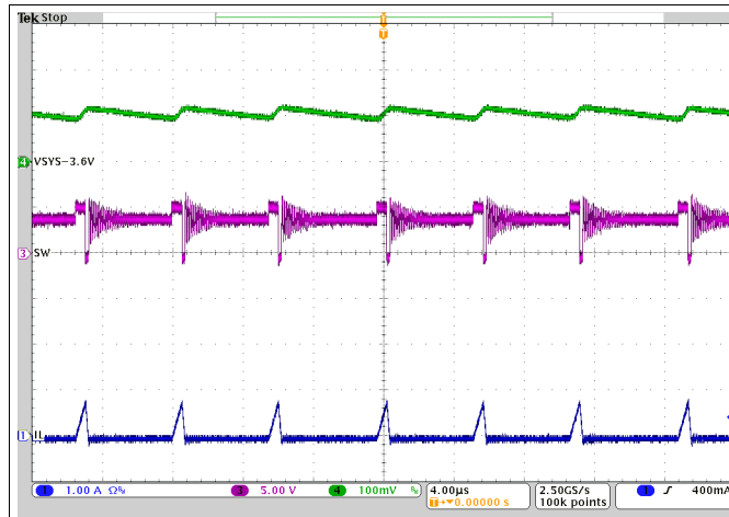
Figure 20. PFM Switching in Buck Mode
