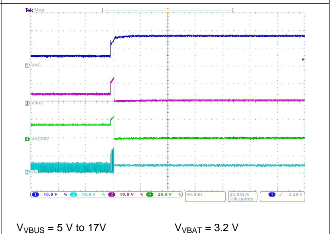
Figure 17. Power-Up with Charge Enabled
