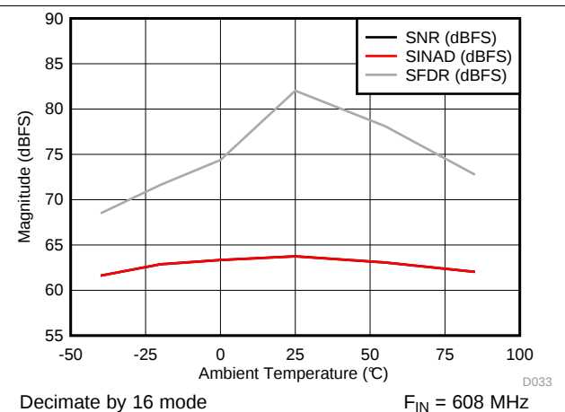
Figure 6. SNR, SINAD, SFDR vs Temperature
