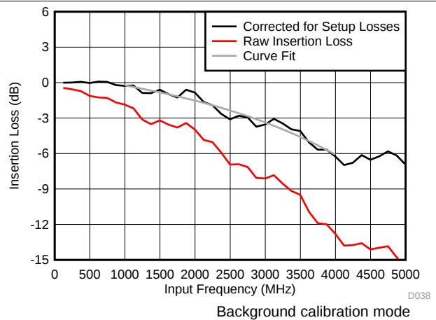
Figure 18. Insertion Loss vs Input Frequency
