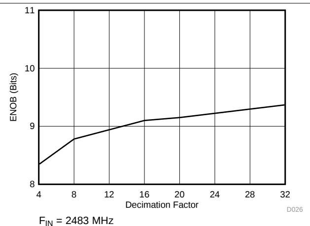
Figure 8. ENOB vs Decimation Setting
