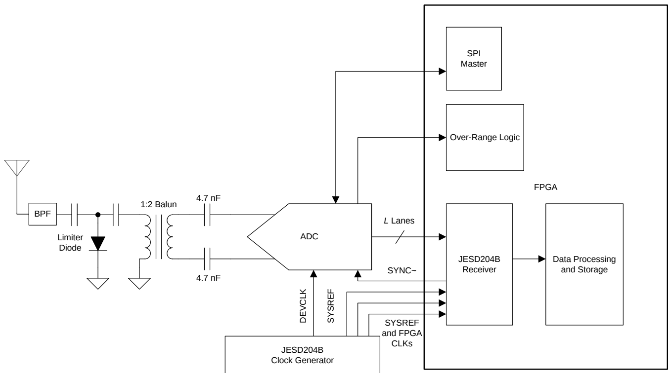
图 77. Simplified Schematic
