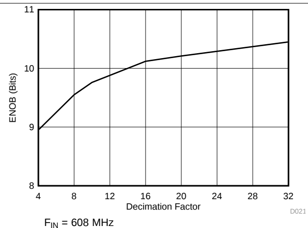
Figure 7. ENOB vs Decimation Setting
