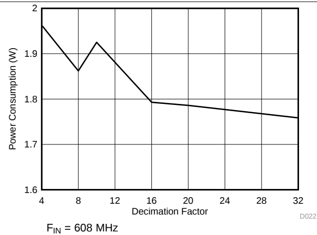
Figure 11. Power Consumption vs Decimation Setting
