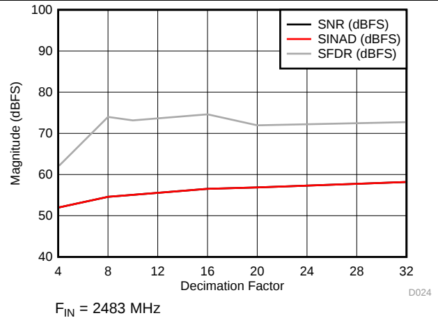
Figure 4. SNR, SINAD, SFDR vs Decimation Setting
