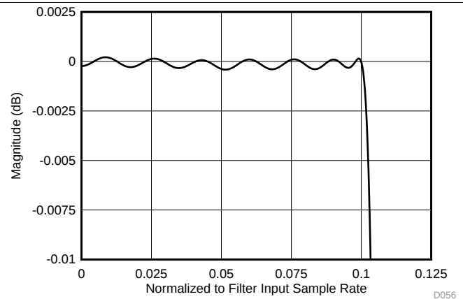
Figure 18. Insertion Loss vs Input Frequency
