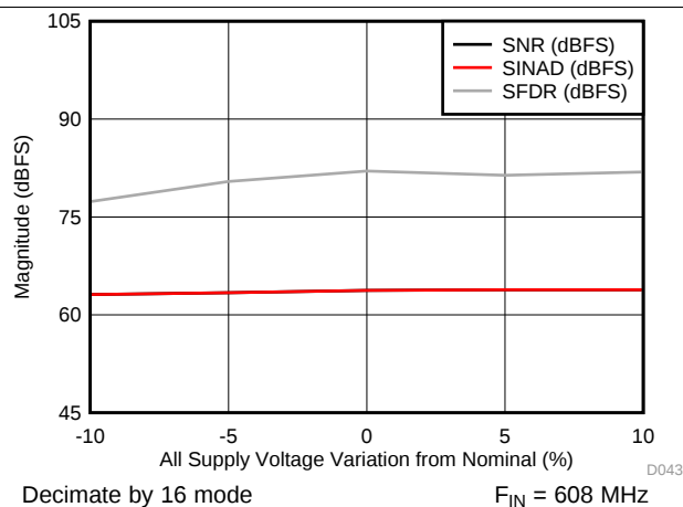
Figure 5. SNR, SINAD, SFDR vs Supply
