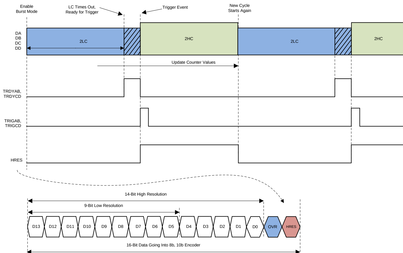
图 59. Timing Diagram for Manual Trigger Mode
