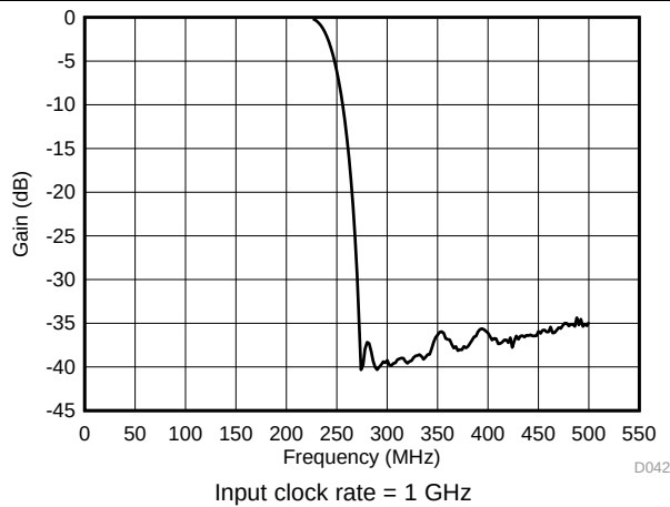
图 47. Decimation Filter Response vs Frequency
