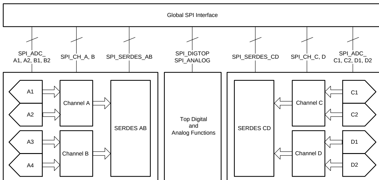
图 74. SPI Register Block Diagram
