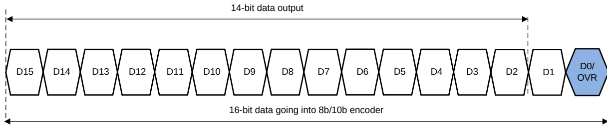
图 61. Timing Diagram for FOVR
