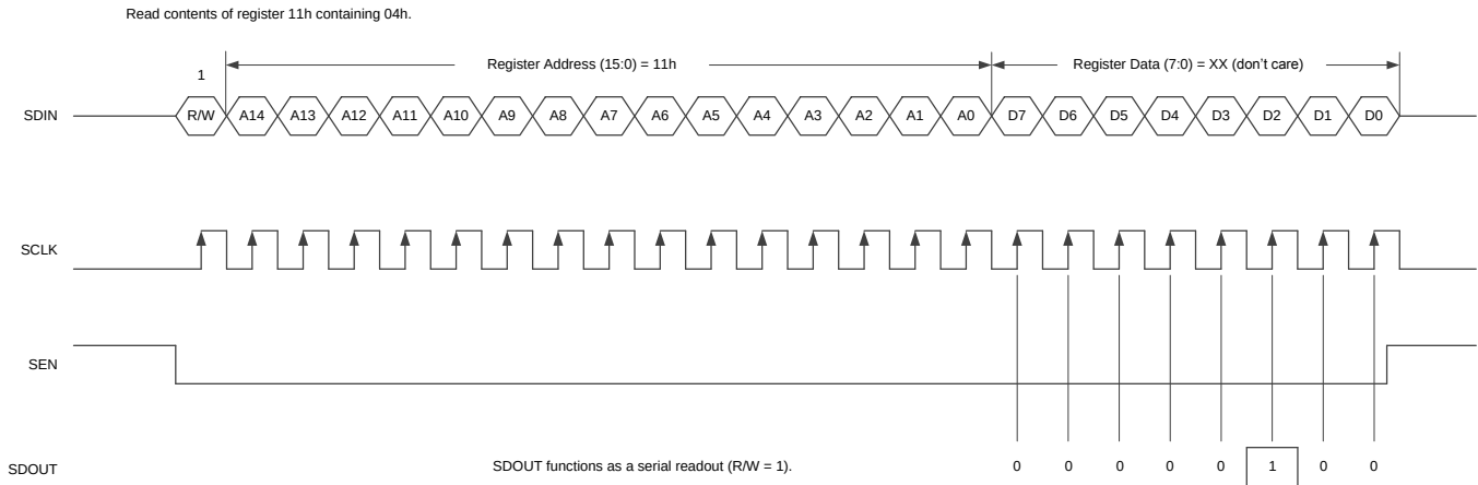
图 73. Serial Interface 4-Wire Read Timing Diagram
