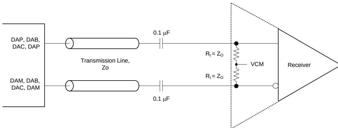
图 67. SerDes Transmitter Connection to Receiver
