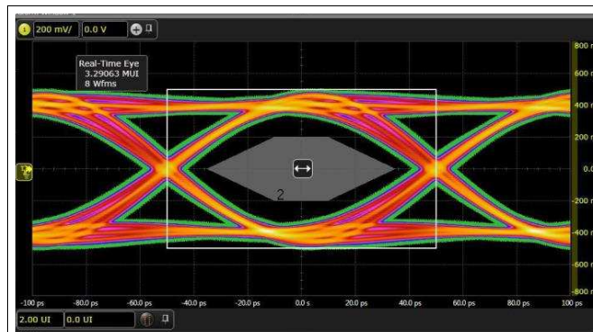
图 68. Eye at 10-Gbps Bit Rate with Default Output Swing
