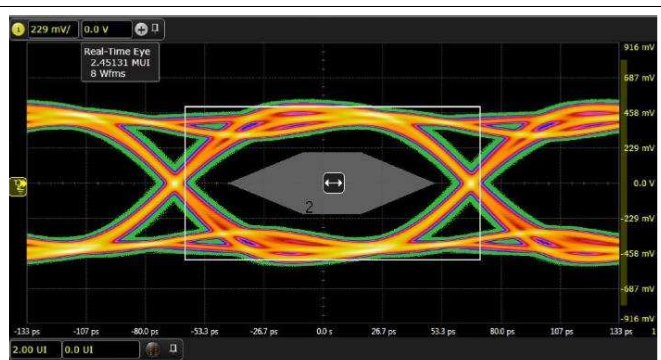
图 69. Eye at 7.5-Gbps Bit Rate with Default Output Swing
