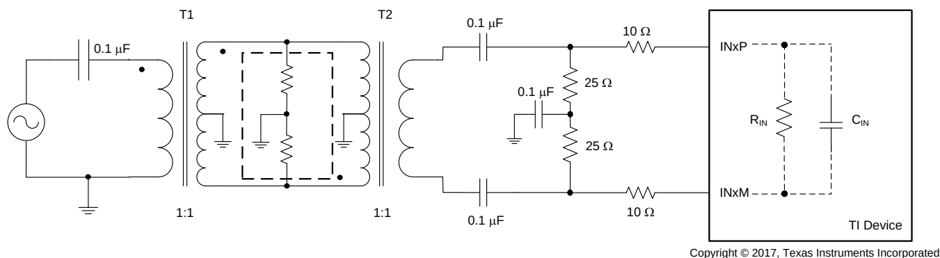
图 43. Analog Input Driving Circuit
