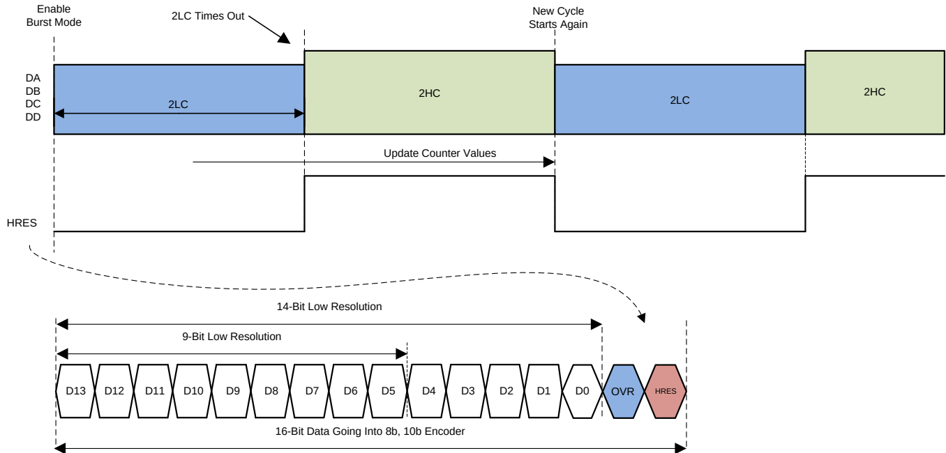
图 60. Timing Diagram for Auto Trigger Mode
