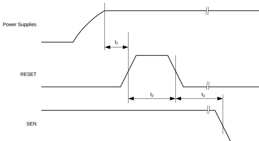
图 132. Hardware Reset Timing Diagram
