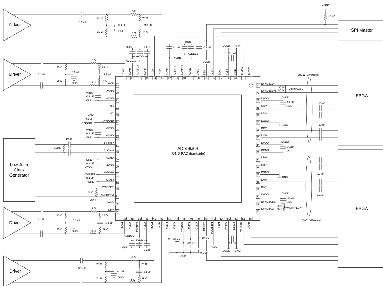
图 135. Application Diagram for the ADS58J64
