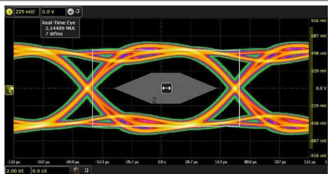
图 71. Eye at 7.5-Gbps Bit Rate with Increased Output Swing
