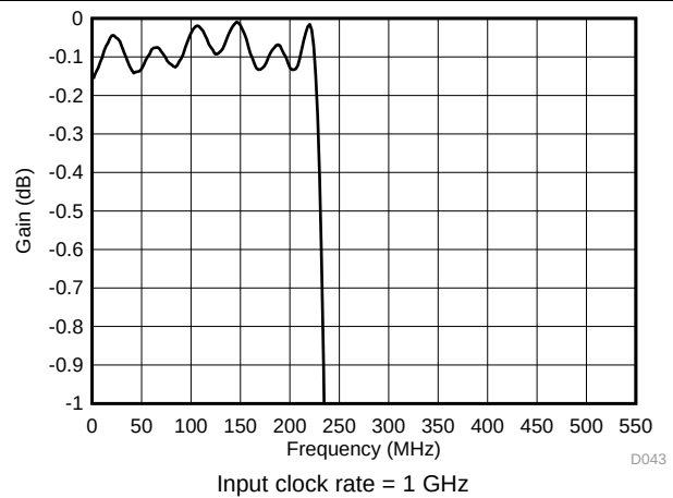
图 48. Decimation Filter Pass-Band Ripple vs Frequency
