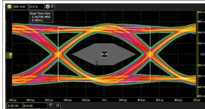
图 70. Eye at 10-Gbps Bit Rate with Increased Output Swing
