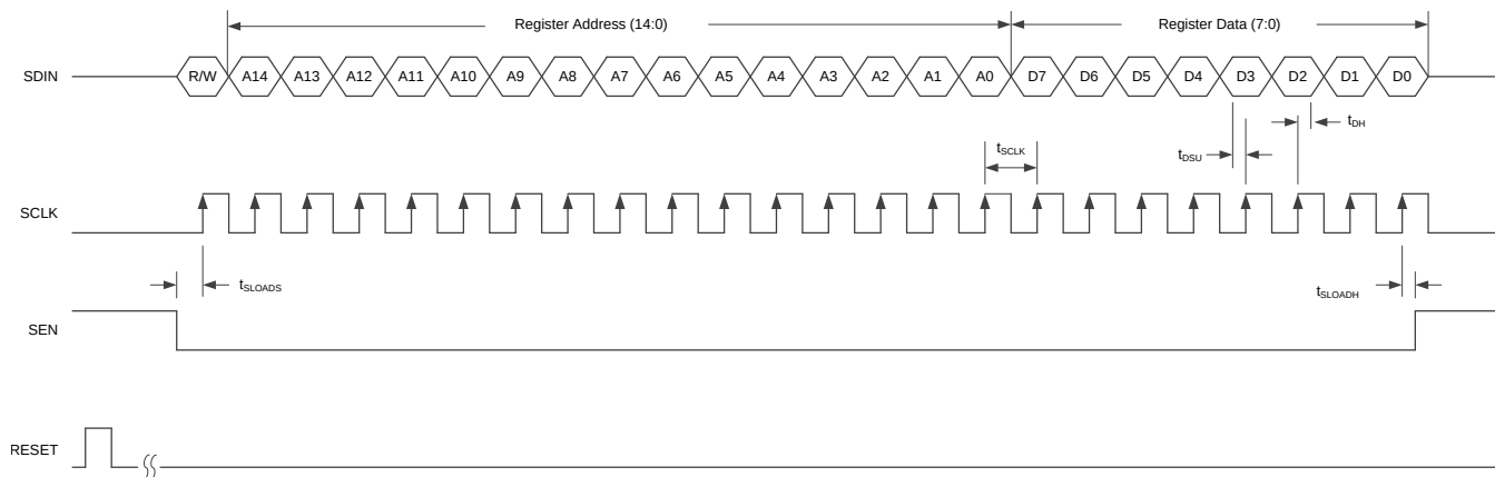
图 72. Serial Interface Write Timing Diagram
