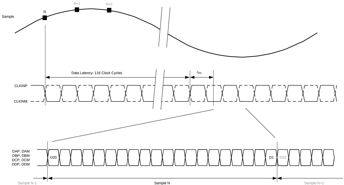
图 1. Latency Timing Diagram in Burst Mode
