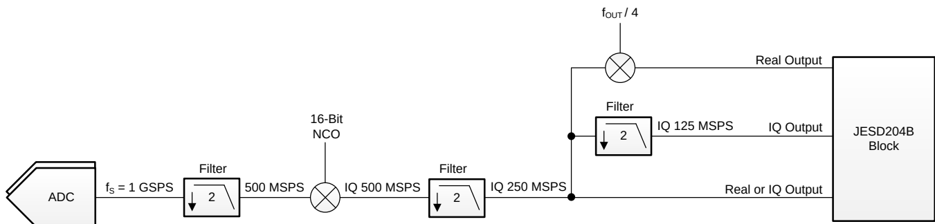
图 46. ADS58J64 Channel (1 of 4) Block Diagram
