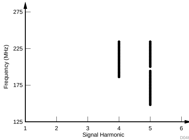
图 133. In-Band Harmonics for a Frequency Planned System
