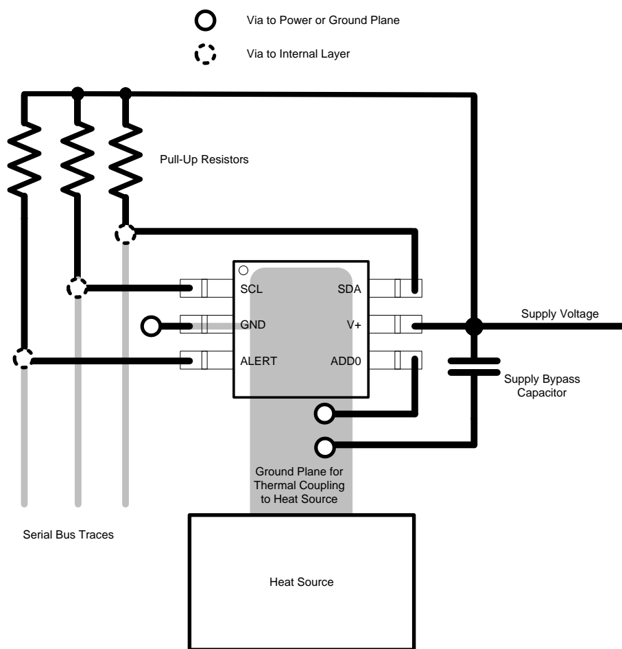
Figure 20. Layout Example
