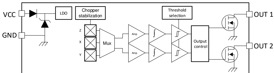
Figure 8-1. Block Diagram
