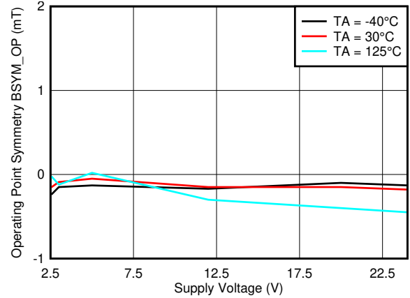
Figure 7-26. B_{SYM\_OP(ZX)} vs. V_{CC}
