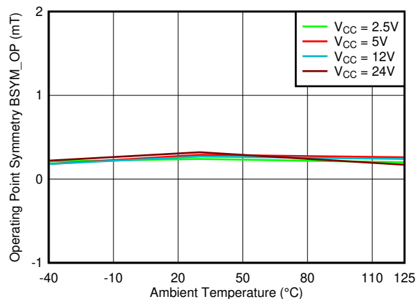
Figure 7-29. B_{SYM\_OP(ZY)} vs. Temperature
