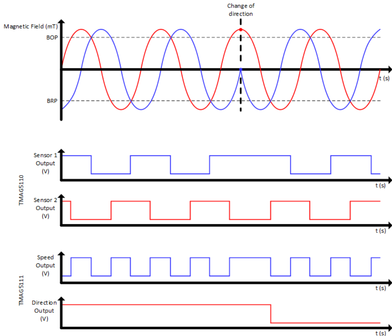
Figure 8-4. TMAG511x Output Behavior
