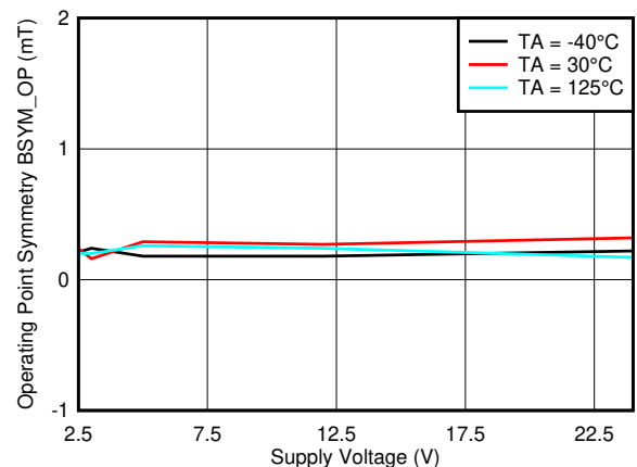
Figure 7-30. B_{SYM\_OP(ZY)} vs. V_{CC}
