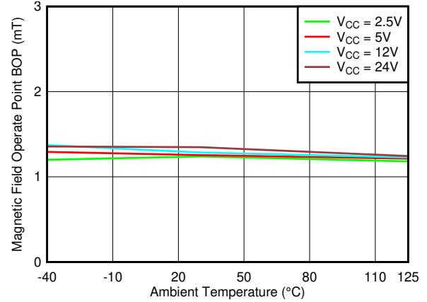
Figure 7-2. B_{OP\_Z} Threshold vs. Temperature
