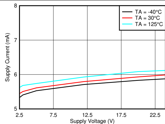
Figure 7-34. Supply Current vs. V_{CC}
