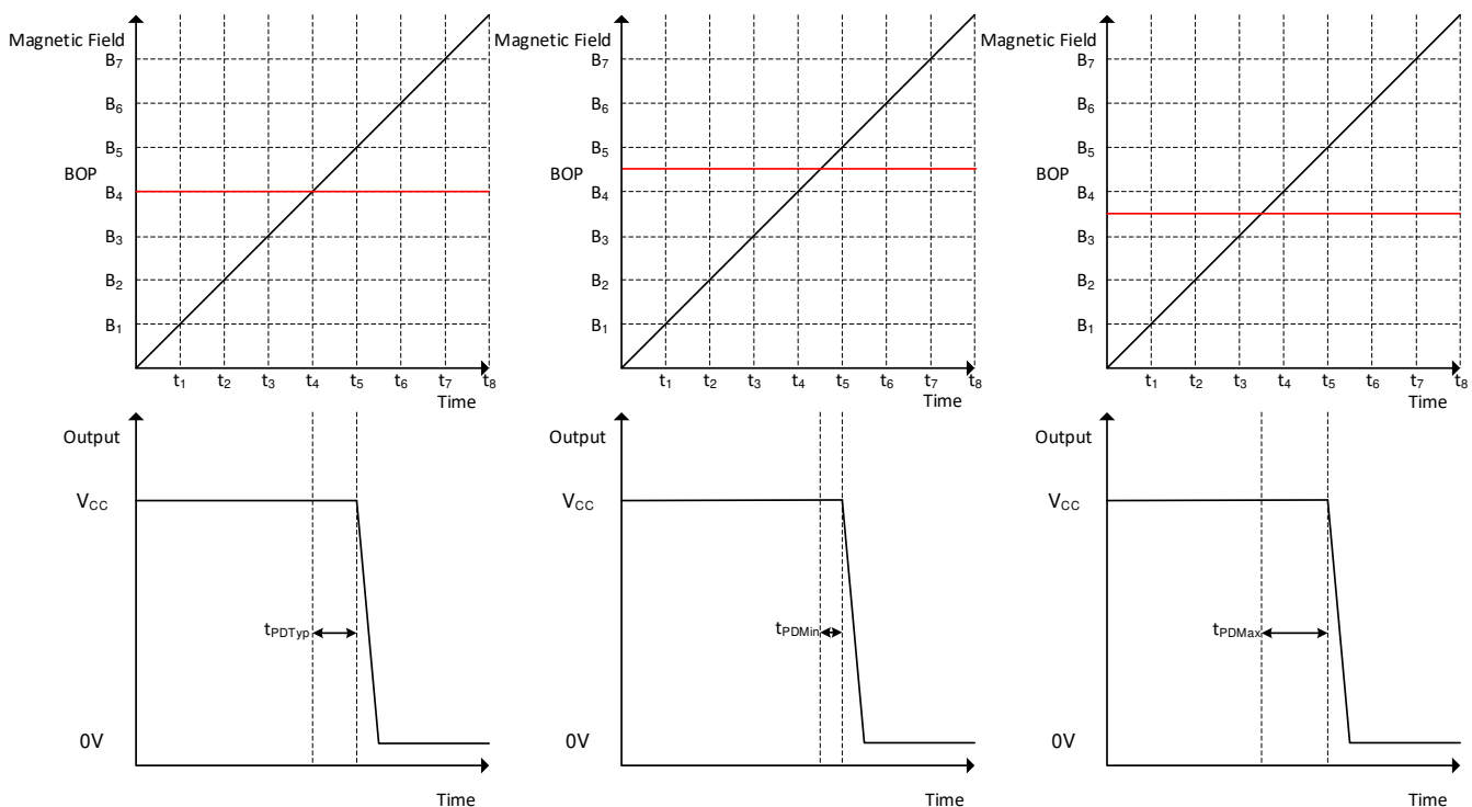
Figure 8-20. Field Sampling Timing
