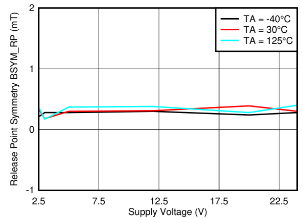
Figure 7-27. B_{SYM\_RP(ZX)} vs. V_{CC}
