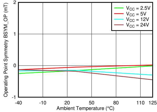
Figure 7-25. B_{SYM\_OP(ZX)} vs. Temperature
