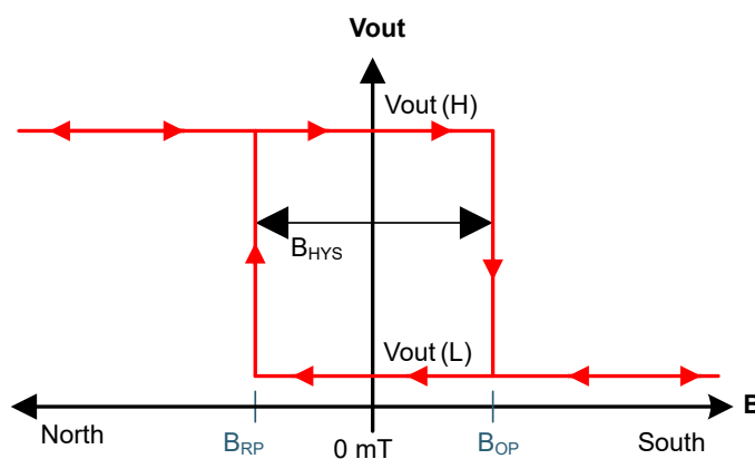
Figure 8-3. Latch Functionality
