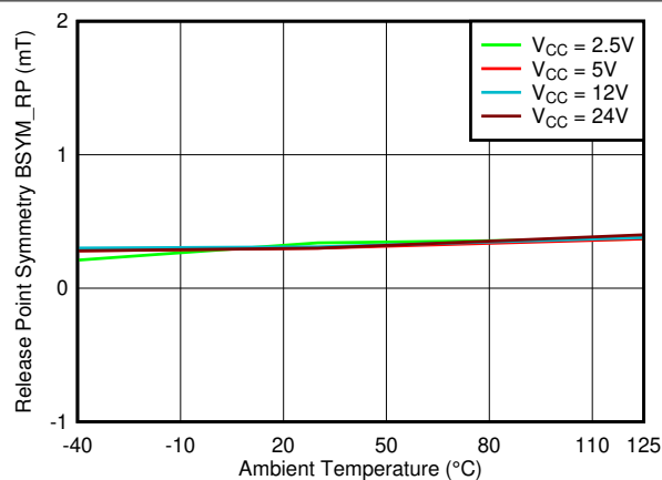
Figure 7-31. B_{SYM\_RP(ZY)} vs. Temperature
