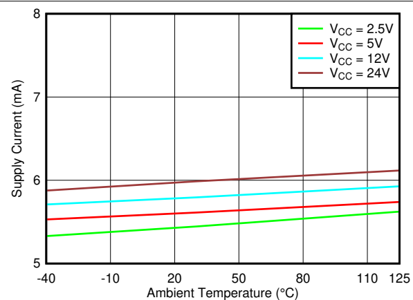
Figure 7-33. Supply Current vs. Temperature
