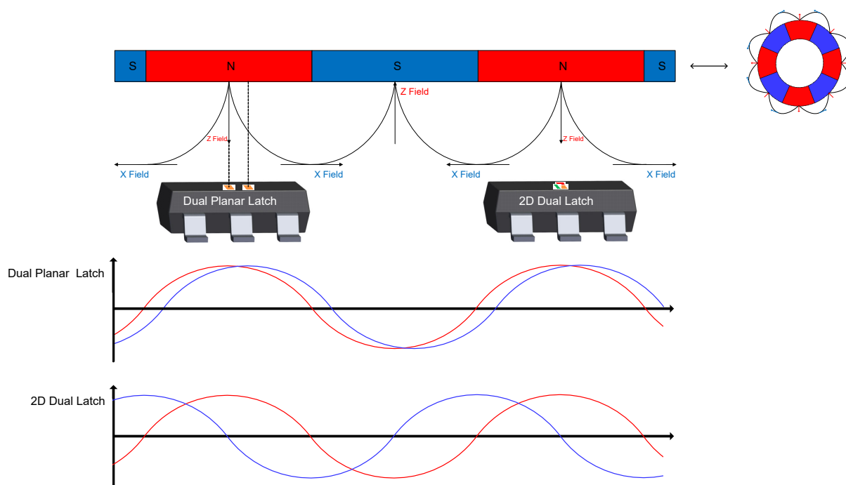
Figure 8-2. Dual Planar Latch vs. 2D Dual Latch
