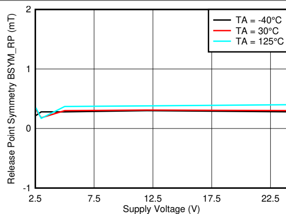
Figure 7-32. B_{SYM\_RP(ZY)} vs. V_{CC}
