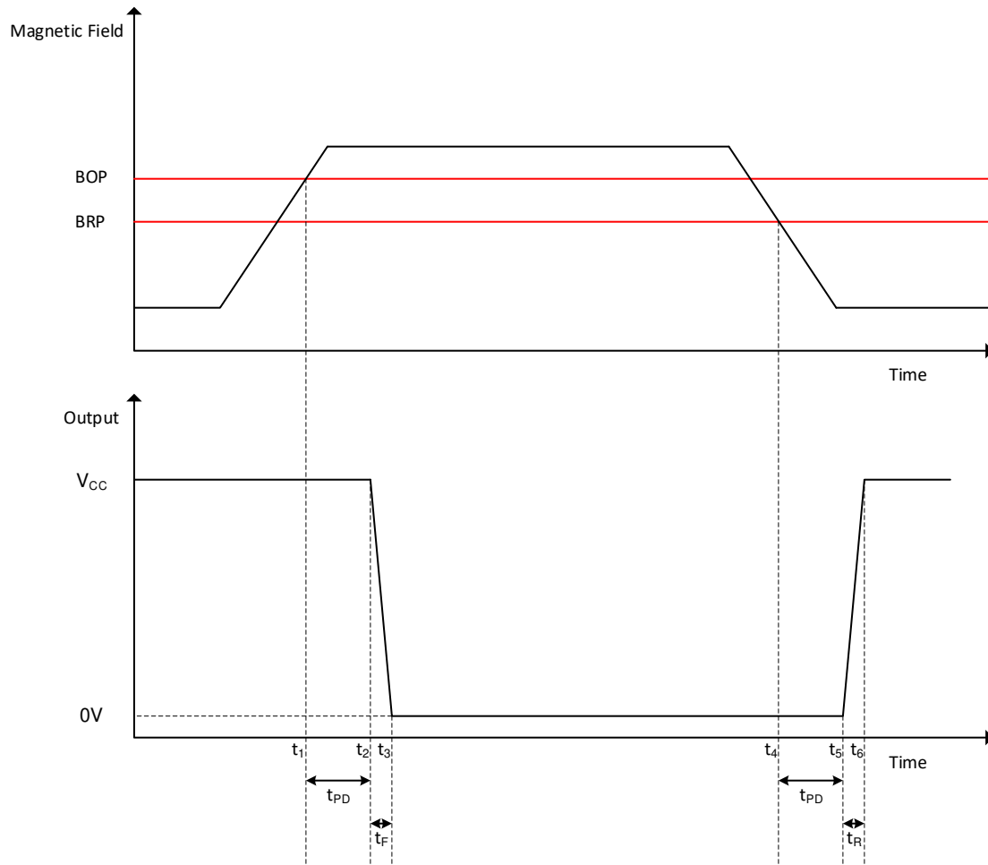
Figure 8-21. Propagation Delay
