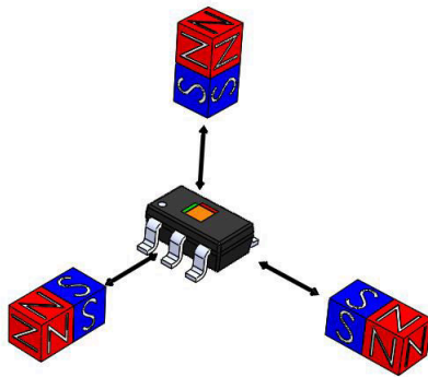
Device Axis Polarities
