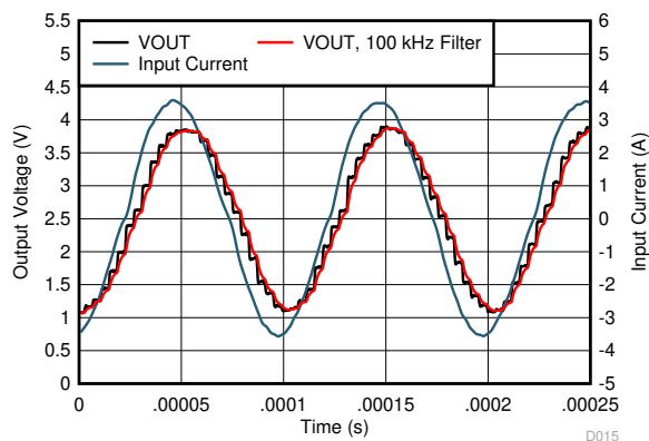
图 9-6. Response Behavior to 10\text{ kHz} Sine Wave Input Current
