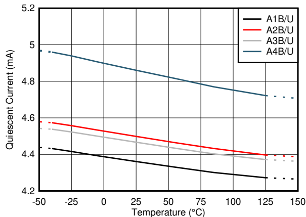
图 7-7. Quiescent Current vs Temperature
