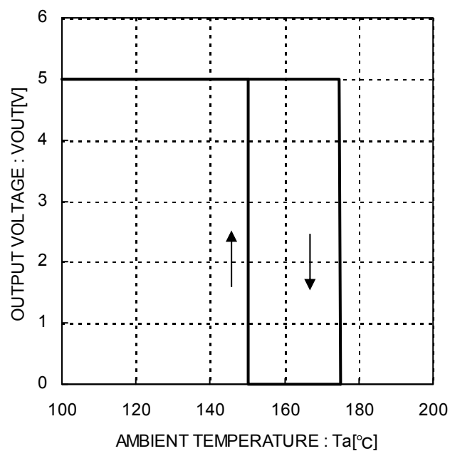
Figure 12. Thermal Shutdown Circuit Characteristics
