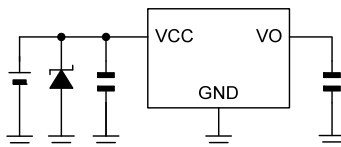
Figure 20. Application Examples 1
