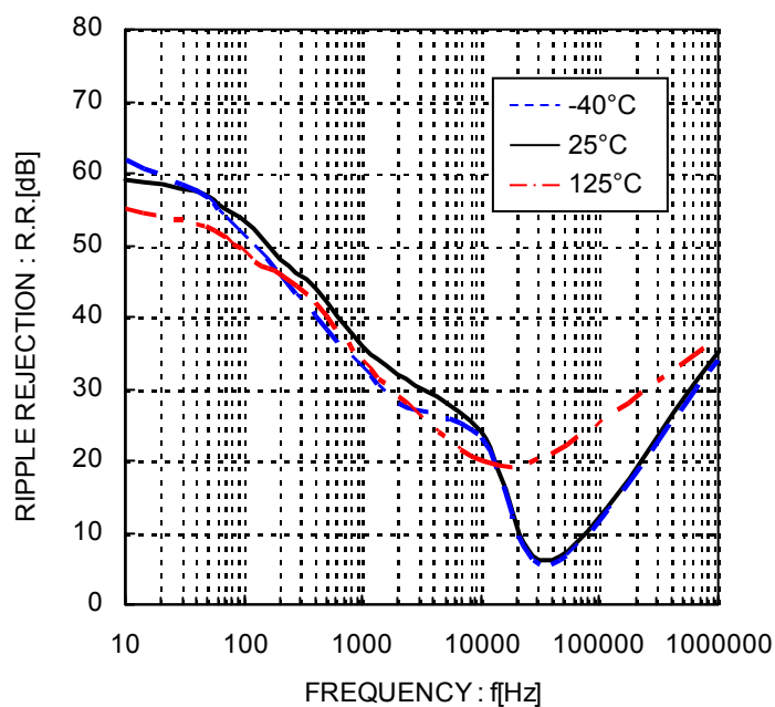
Figure 10. Ripple Rejection
