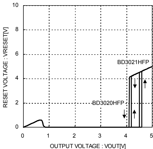
Figure 13. Detection Voltage ( V_{CC}=V_{OUT} )
