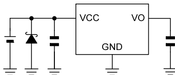
Figure 21. Application Examples 2
