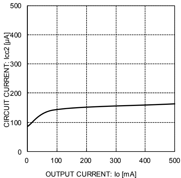
Figure 6. Circuit Current 2
