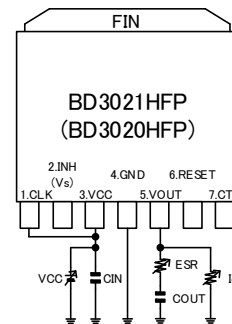
*Pin Settings / Precautions2 Measurement circuit
