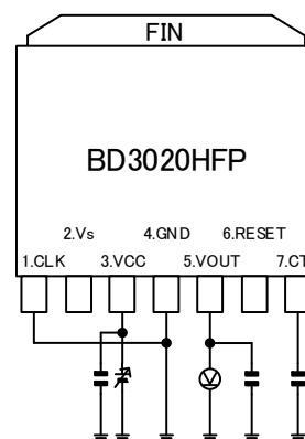
Measurement setup for Figure 7, 11, 12.
