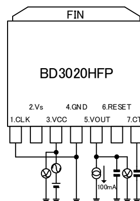
Measurement setup for Figure 10.
