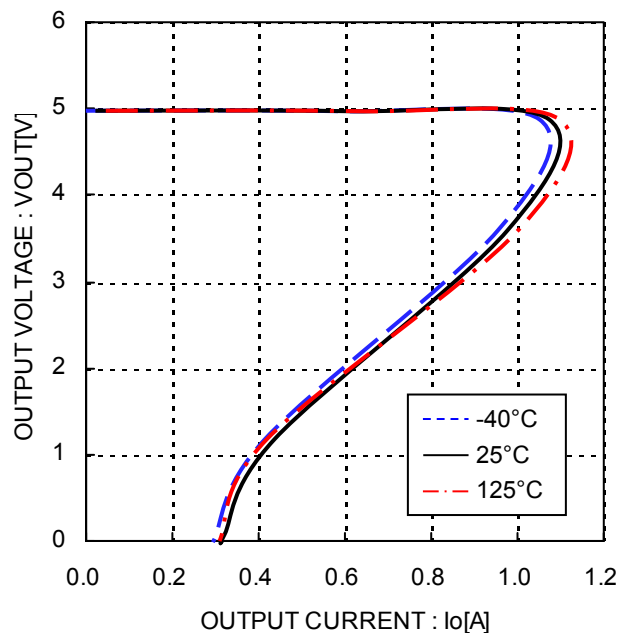
Figure 8. Load Stability
