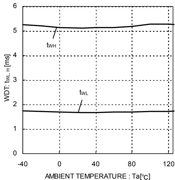
Figure 16. WDT Time vs. Temperature ( C_{CT}=0.01\mu\text{F} )
