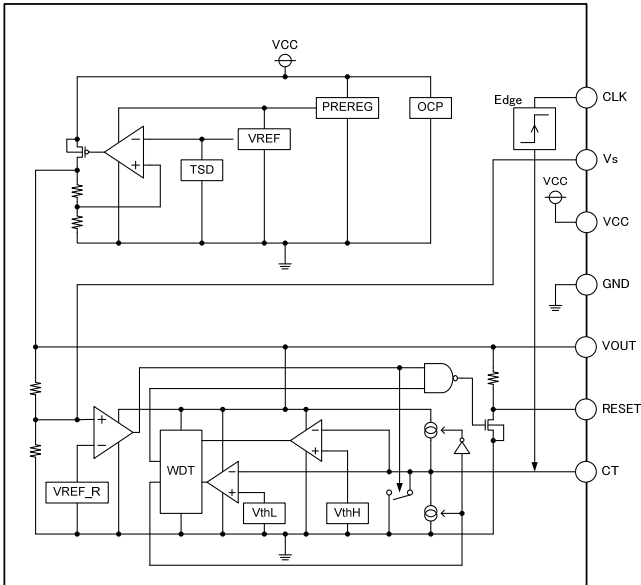
Figure 4. Block Diagrams
