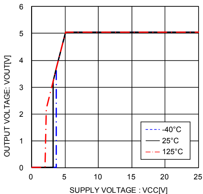
Figure 7. Input Stability
