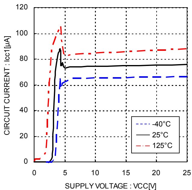
Figure 5. Circuit Current 1
