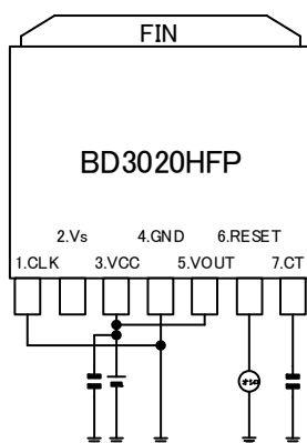
Measurement setup for Figure 16.
