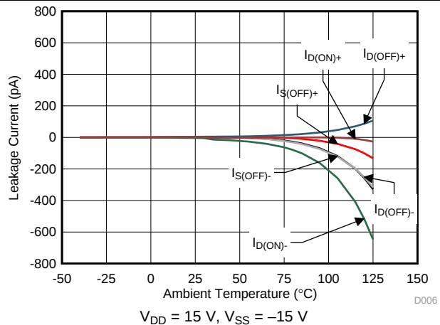
图 6. Leakage Current vs Temperature
