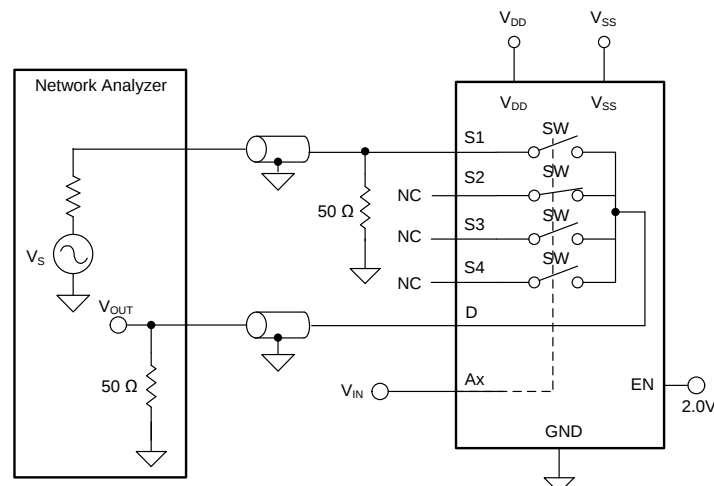
图 24. Off Isolation Measurement Setup
