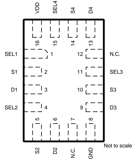
RSV Package 16-Pin QFN Top View
