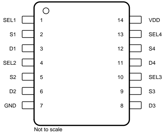
PW Package 14-Pin TSSOP Top View
