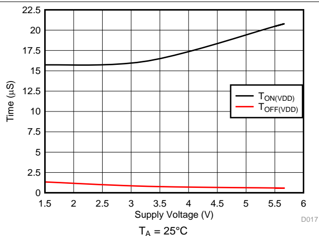
图 17. T_{ON}(VDD) and T_{OFF}(VDD) vs Supply Voltage
